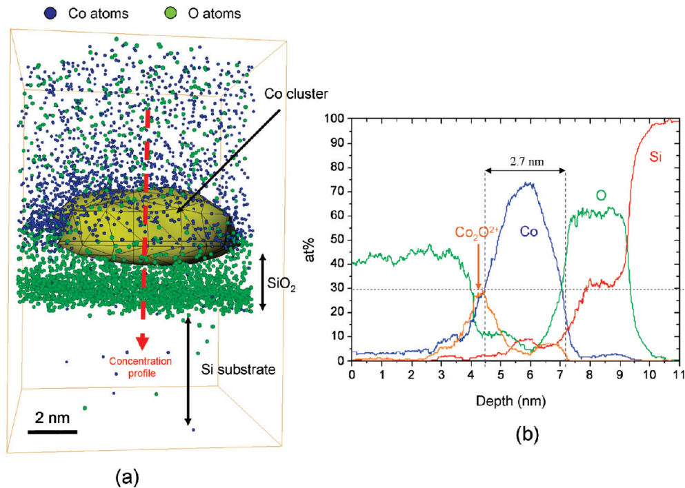
Figure 7. (a) 3D image of a Co cluster grown on the SiO 2 layer (in yellow, iso-concentration surface at 30 Co at. %); (b) concentration profile through the Co cluster along the red arrow in (a).
