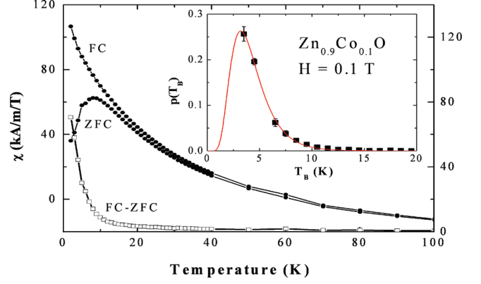
Figure 4. Zero-field-cooled/field-cooled magnetization curves (●) obtained on the \text{Zn}_{0.9}\text{Co}_{0.1}\text{O} thin film with an applied magnetic field of 1 kOe. In the inset is shown the blocking temperature distribution estimated from the derivative of the difference of the ZFC/FC curves (□) divided by T (■) and its adjustment as a log-normal distribution.
