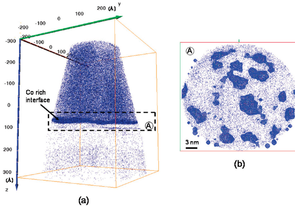
Figure 6. (a) Distribution of Co atoms in the analyzed volume of Zn 0.9 Co 0.1 O; (b) top view of the Zn(Co)O/SiO 2 interface: the inhomogeneous distribution of Co atoms is evidenced by iso-concentration filter (threshold: 40% of Co).
