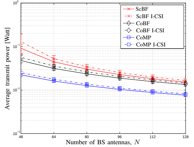
Fig. 6. Average transmit power in Watt vs. N when L = 16, K = 8 and the rates are randomly taken in the interval [1, 3] .
