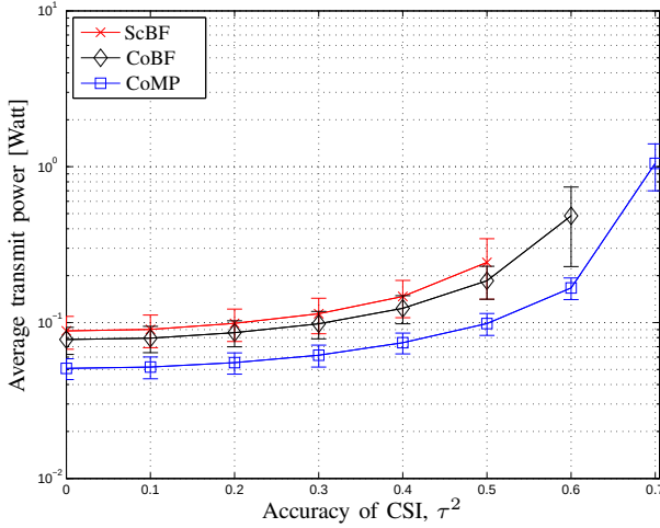
Fig. 4. Average transmit power in Watt vs. \tau^2 when L = 4, K = 8, N = 32 and r = 2 [bps/Hz/UE].
