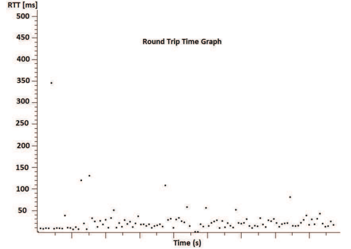
Fig. 6: Round Trip Time Between Client and a Fog Server
