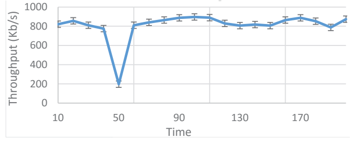
Fig. 8: TCP Throughput
