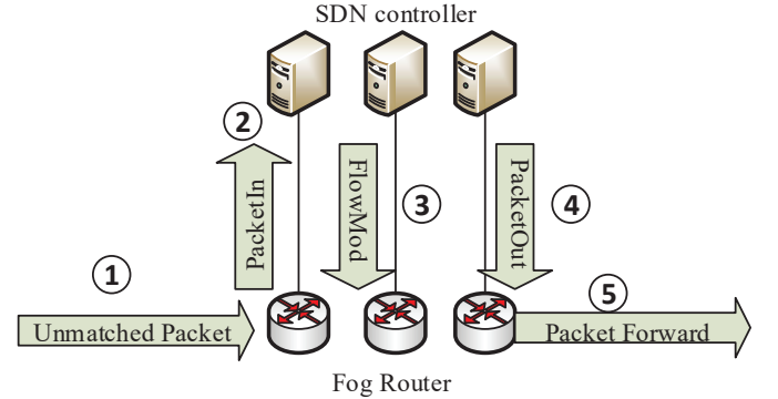
Fig. 4: Installation Procedure of a new flow
