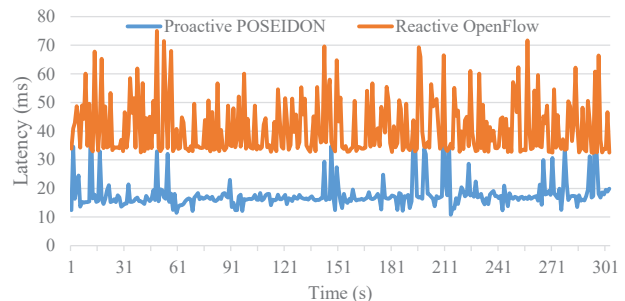
Figure 9: Latency: Proactive POSEIDON vs. Reactive OpenFlow
