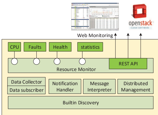
Figure 4: Monitoring node
