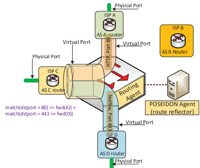
Figure 8: Transforming the underlying topology into single virtual switch
