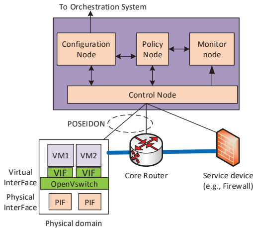
Figure 2: Internal components of the POSEIDON Agent
