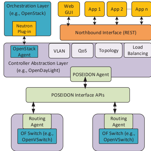
Figure 1: POSEIDON Architecture
