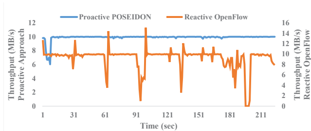
Figure 10: Efficient Bandwidth usage for POSEIDON
