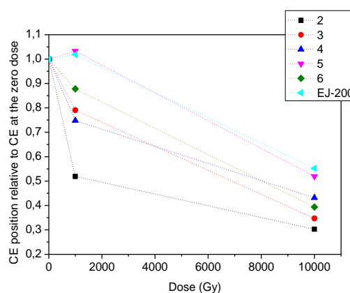
Figure 6. Evolution of the CE position relative to the initial value at different irradiation doses for samples 2 – 6 and EJ-200 plastic scintillator. The lines are drawn to guide the eye.
