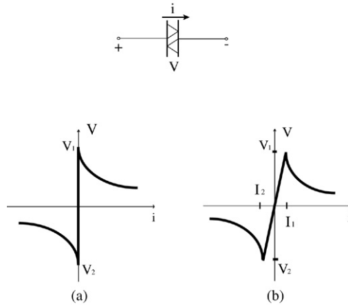
Fig. 5. Diac model.
