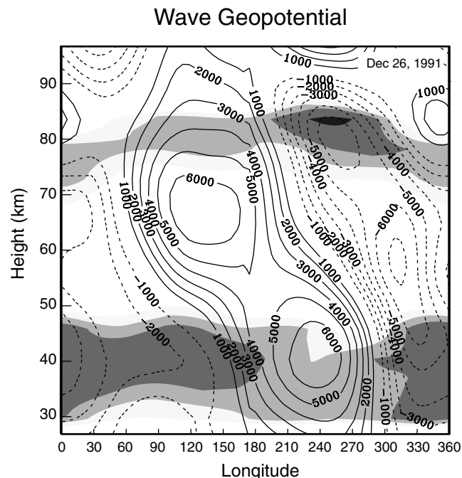
Figure 7. As in Figure 6, but on 26 December 1991.
