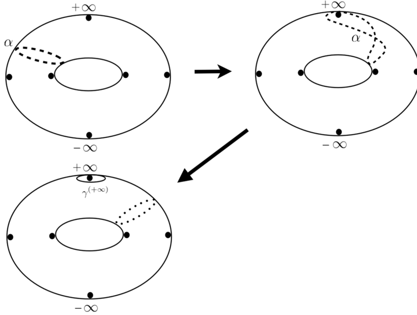
Figure 6. Deformation of the \alpha loop in the left well. It splits into a combination of the \alpha loop in the right well and a loop around +\infty .
