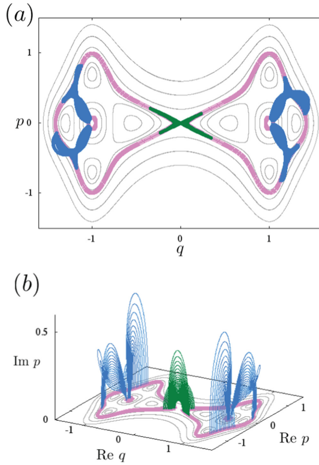
Figure 14. (a) Equi-energy contours for the Hamiltonian (36). The magenta curves show energy contours satisfying the condition E \sim E_n^\pm where E = 6.19 \times 10^{-3} . The blue curves are projections onto the real plane of complex manifolds connecting inside and outside energy contours. The green one shows projection of complex manifolds connecting left and right outer energy contours. (b) The projection of each manifold onto (\text{Re } q, \text{Re } p, \text{Im } p) space.
