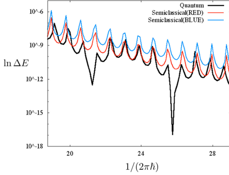
Figure 13. The tunnelling splitting \Delta E_n = E_n^- - E_n^+ as a function of 1/\hbar . Here E_n^+ \simeq E_n^- \simeq E = 6.19 \times 10^{-3} . The black curve shows the numerical result obtained by direct calculation. The blue and red ones are obtained by applying the semiclassical formula (44), and the corresponding time paths are respectively shown in figure 16.
