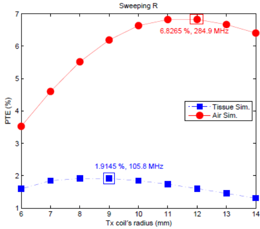
Figure 3 : PTE simulation results in CST for 24mm-diameter Tx coil radii, in presence or not of the muscle tissue influence.
