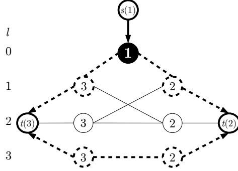
FIG. 6. Graph \overline{\mathbf{G}}(w, y) = (\overline{\mathbf{V}}(w), \overline{\mathbf{E}}(w, y)) associated to the second extreme point (w, y) depicted in Figure 4 and considering demands (1, 2) and (1, 3). Thin edges (resp. nodes) correspond to the components of y (resp. w ) equal to zero and do not belong to \overline{\mathbf{E}}(w, y) (resp. \overline{\mathbf{V}}(w) ).
