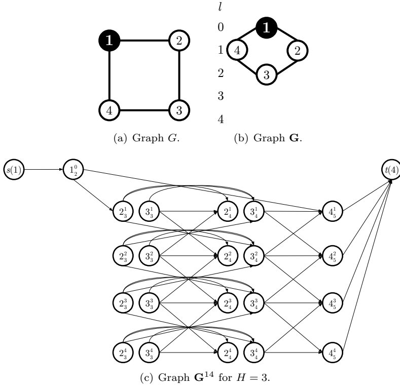
FIG. 8. Hop-level graph.
