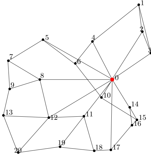
FIG. 1. Optimal solution of a HSNBP instance with K = 3 and H = 3 ; n = 21 , D = \{(0, v) : v = 1, \dots, 20\} , complete graph, Euclidean costs.
