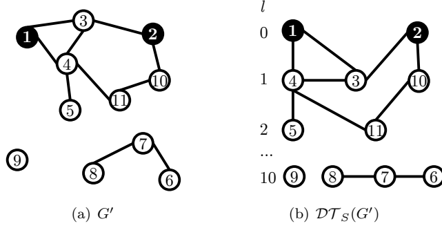
FIG. 2. Original graph G' and \mathcal{DT}_S(G') with S = \{1, 2\} .
