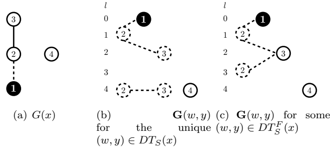
FIG. 7. Example of fractional x , the single point in DT_S(x) , and a point in DT_S^F(x) ( S = \{1\} ).
