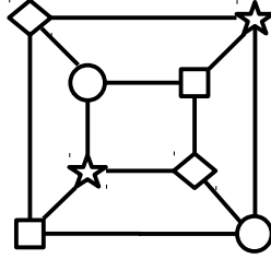
FIG. 10. STF instance with 4 demands (pairs of identical symbols), unitary edge costs.
