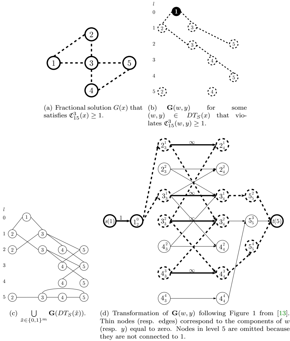
FIG. 9. Separation of 3-path cut inequalities following [13].
