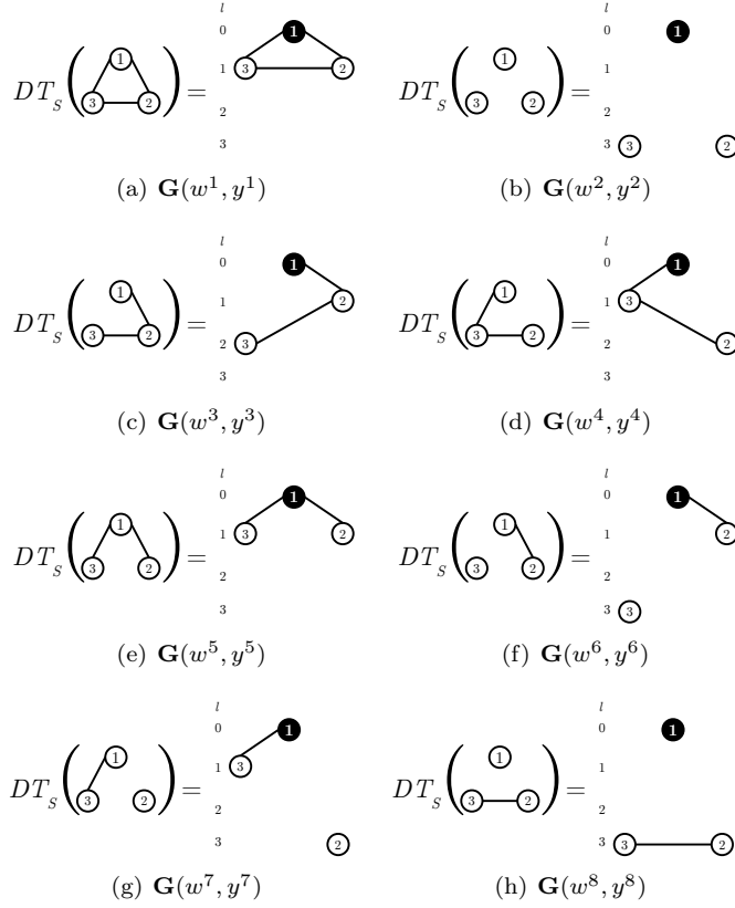
FIG. 3. Graph induced by DT_S^{int}(x) for each x \in \{x^1, \dots, x^8\} = \{0, 1\}^3 .
