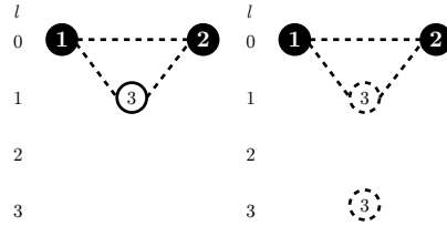
FIG. 5. Examples of graphs induced by the elements of \text{ext}(DT_S(\bar{x})) when S = \{1, 2\} .
