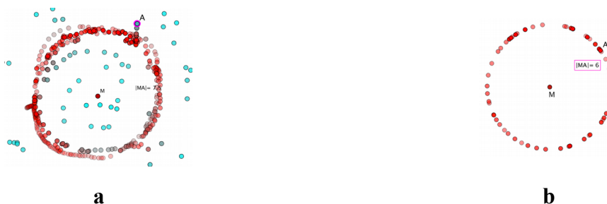
Fig. 3: Circle as a locus of points that are at a given distance from a given point: (a) “soft” locus, and (b) “robust” locus.
