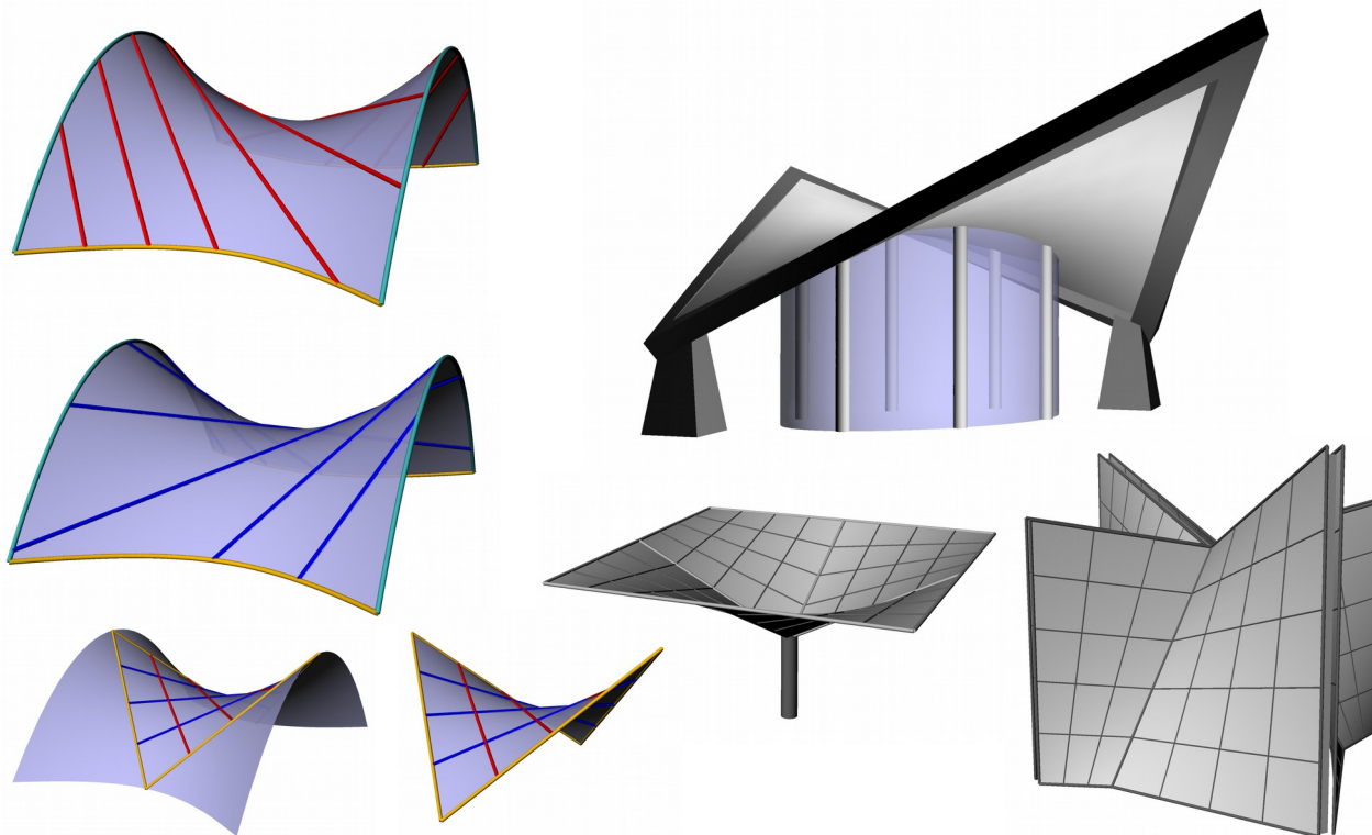
Figure 1: Ruled surfaces - determination and practical applications.
