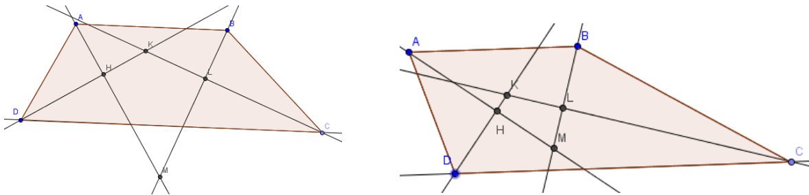
Figure 7. Constructing a robust trapezoid and dragging to identify invariants
