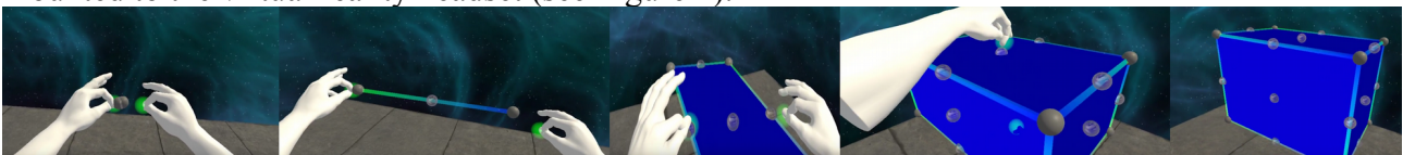
Figure 1. Different cases of the stretch operator: a point is stretched into a line segment, the segment is stretched into a plane figure, and the plane figure is stretched into a prism.
