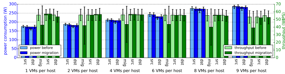
Figure 8: Overheads upon VM migration.
