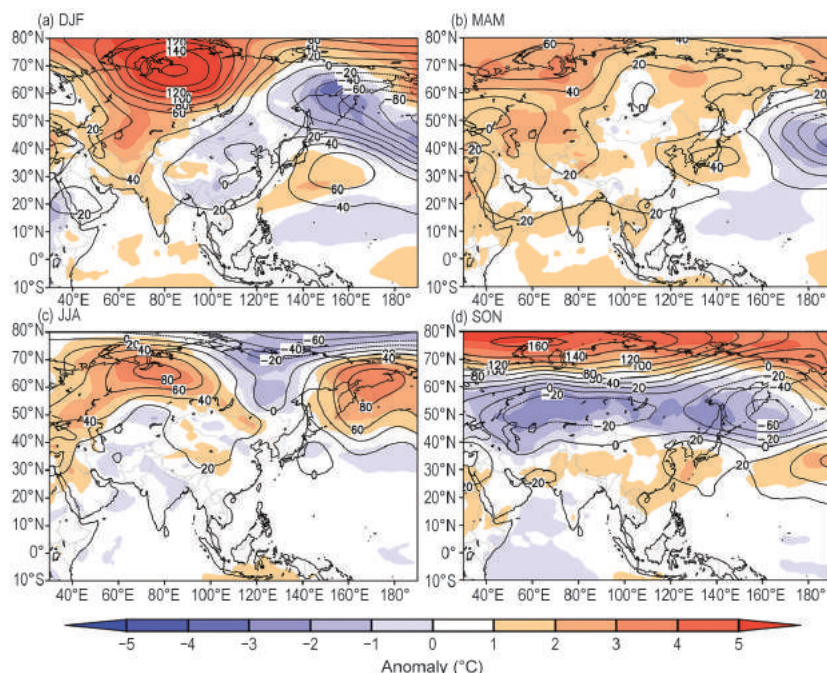
FIG. 7.44. Seasonal mean anomalies of 500-hPa geopotential height (contour, gpm) and 850-hPa temperature (shading, ^\circ\text{C} ) for (a) winter, (b) spring, (c) summer, and (d) autumn, using data from the JRA-55 reanalysis. The base period is 1981–2010. (Source: Japan Meteorological Agency.)
