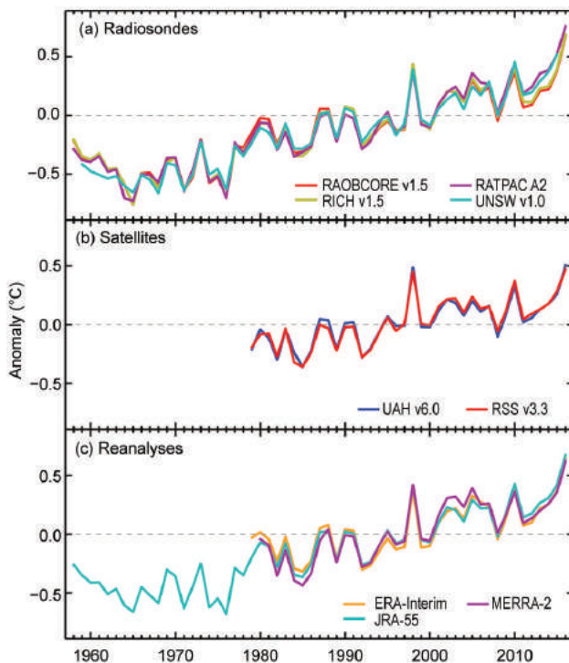
FIG. 2.6. Global average lower tropospheric temperature annual anomalies ( ^\circ\text{C} ; 1981–2010 base period for the MSU LT equivalent layer). (a) Radiosonde: RATPAC (Free et al. 2005), RAOBCORE and RICH (Haimberger et al. 2012) and UNSW (Sherwood and Nishant 2015). (b) Satellites: UAHv6.0 (Spencer et al. 2017) and RSSv3.3 (Mears and Wentz 2009). (c) Reanalyses: ERA-Interim (Dee et al. 2011), MERRA-2 (Bosilovich et al. 2015; Gelaro et al. 2017), and JRA-55 (Ebita et al. 2011; Kobayashi et al. 2015).
