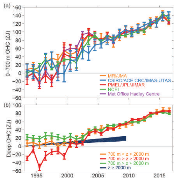
FIG. 3.6. (a) Annual average global integrals of in situ estimates of upper (0–700 m) OHCA (ZJ; 1 \text{ ZJ} = 10^{21} \text{ J} ) for 1993–2016 with standard errors of the mean. The MRI/JMA estimate is an update and modification of Ishii and Kimoto (2009). The CSIRO/ACE CRC/IMAS-UTAS estimate is an update of Domingues et al. (2008). The PMEL/JPL/JIMAR estimate is an update and refinement of Lyman and Johnson (2014). The NCEI estimate follows Levitus et al. (2012). The Met Office Hadley Centre estimate is computed from gridded monthly temperature anomalies (relative to 1950–2016) following Palmer et al. (2007). See Johnson et al. (2014) for details on uncertainties, methods, and datasets. For comparison, all estimates have been individually offset (vertically on the plot), first to their individual 2005–16 means (the best sampled time period), and then to their collective 1993 mean. (b) Annual average global integrals of in situ estimates of intermediate (700–2000 m) OHCA for 1993–2016 with standard errors of the mean, and a long-term trend with one standard error uncertainty shown from 1992–2009 for deep and abyssal ( z > 2000 \text{ m} ) OHCA updated (Desbruyères et al. 2016) following Purkey and Johnson (2010).
