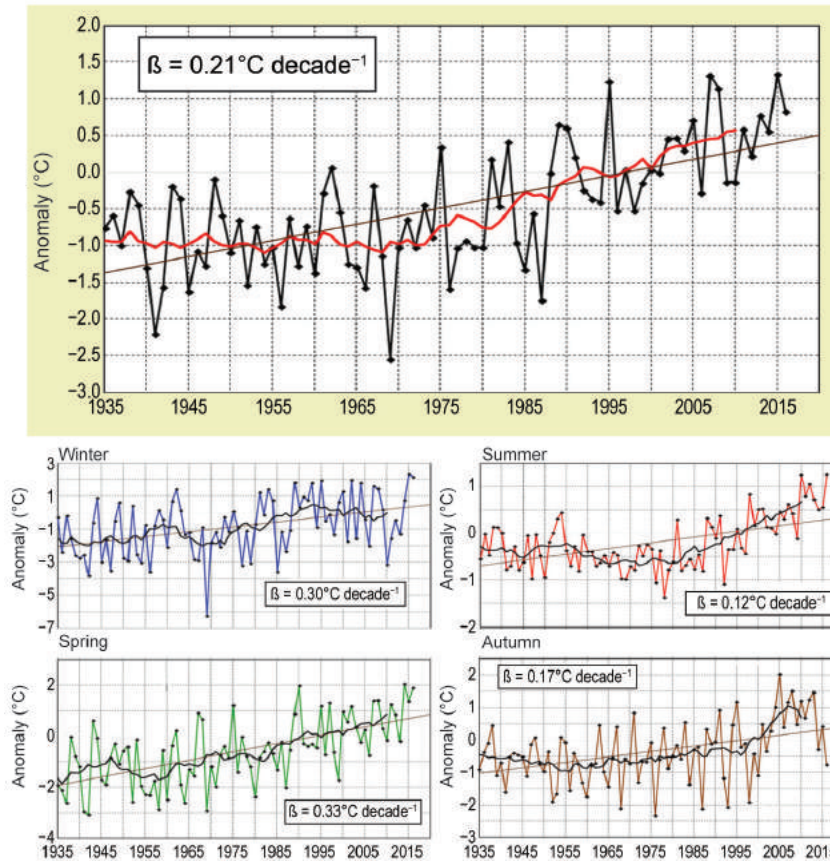
FIG. 7.45. Anomalies of mean (top) annual and (bottom) seasonal air temperatures ( ^{\circ}\text{C} ) averaged over available surface station observations in the Russian territory for the period 1936–2016 (base period: 1981–2010). The 11-year running mean is shown as a continuous line (the time series was “mirrored” before 1936 prior to filtering, but no estimate was made for future years after 2016).
