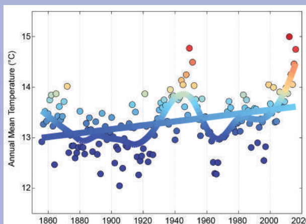
FIG. SB3.1. Mean annual temperature ( ^\circ C , colors) on the northeast U.S. shelf ecosystem ( 36 – 46^\circ N , 76 – 66^\circ W ) derived from the ERSSTv4 dataset ( www.esrl.noaa.gov/psd/data/gridded/data.noaa.ersst.v4.html ). Long-term change is estimated with a linear regression (straight line) and multidecadal variability is estimated with a loess smoother. As depicted, the temperatures, as indicated on the y-axis, transition from dark blue (lowest) to red (highest).
