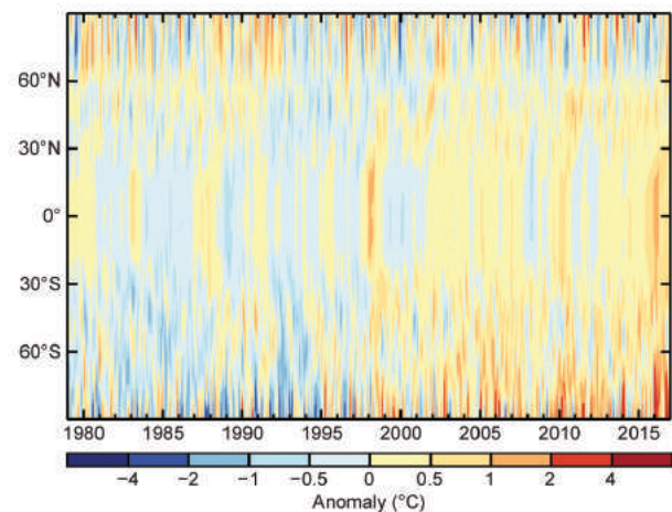
FIG. 2.7. Latitude–time cross-section of lower tropospheric temperature anomalies ( ^\circ\text{C} ) relative to 1981–2010 from ERA-Interim (Dee et al. 2011).
