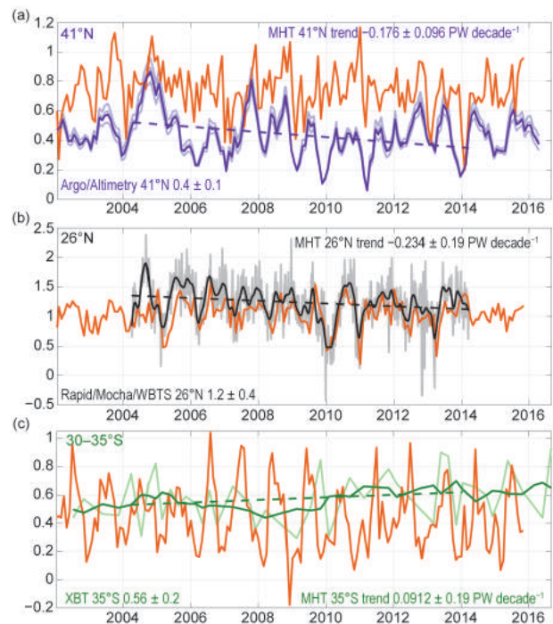
FIG. 3.23. AMHT; (PW) at (a) 41°N (from profiling floats following Hobbs and Willis 2012; blue lines), with uncertainties (light blue lines) and the trend (dashed blue line); at (b) 26°N (from mooring/hydrography data) 12-hourly values (gray line), filtered with a 3-month low-pass filter (black line), and the trend (black dashed line); and at (c) 30°–35°S (from XBTs) quarterly values (light green), filtered with yearly boxcar (dark green line), and the trend (dashed green line). Heat transports simulated by EC (orange lines; Menemenlis et al. 2008) are shown at all latitudes.
