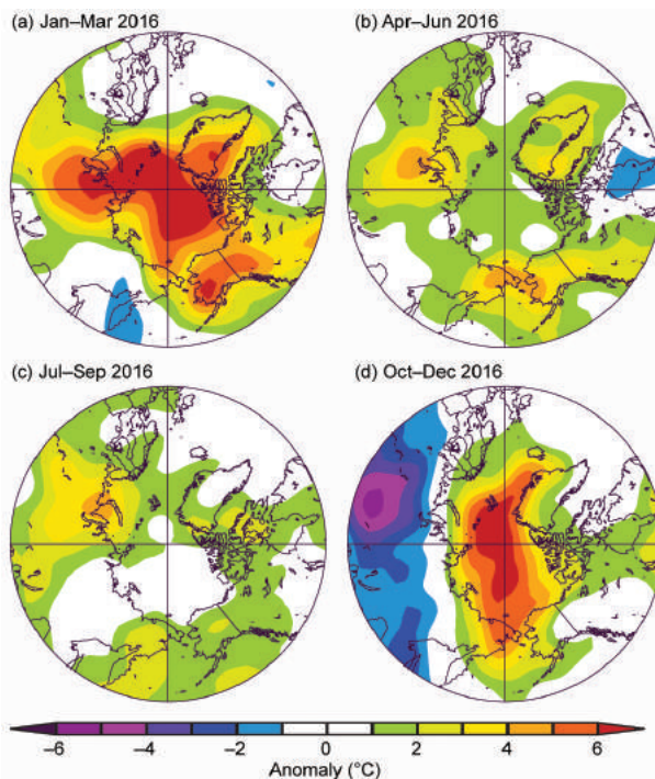
FIG. 5.2. Seasonal anomaly patterns for near-surface air temperatures ( ^{\circ}\text{C} ) in 2016 relative to 1981–2010 in (a) winter (Jan–Mar), (b) spring (Apr–Jun), (c) summer (Jul–Sep), and (d) autumn (Oct–Dec). Temperatures are from slightly above the surface layer (925-mb level) to emphasize large spatial patterns rather than local features. (Source: NOAA/ESRL, www.esrl.noaa.gov/psd/ .)
