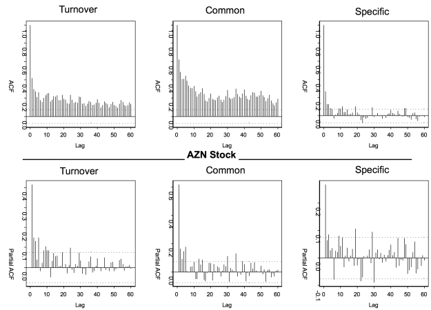
Fig. 7. Autocorrelation and partial autocorrelation functions of the two components, AZN Stock.
