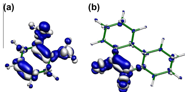
Figure 4. Vibronic coupling densities (VCDs) for effective modes: (a) C 2 symmetrical diamine cation and (b) dione anion. The isosurface values are 2.0 \times 10^{-3} a.u. Blue and gray surfaces are negative and positive contributions, respectively.
