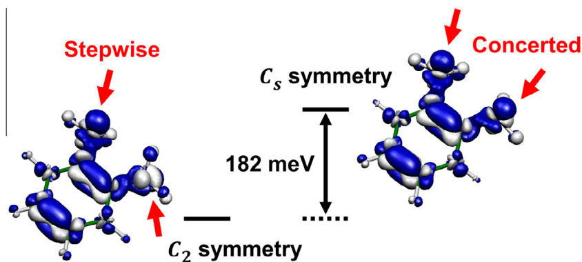
Figure 8. Vibronic coupling densities (VCDs) for effective vibrations of C_2 and C_5 symmetrical diamine cations. Isosurface values are 2.0 \times 10^{-5} a.u. Blue and gray surfaces are stabilizing and destabilizing contributions, respectively. Note that signs on VCD of amino groups differ in the C_2 structure and are the same in the C_5 structure.
