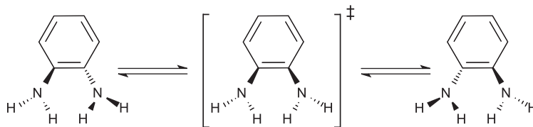
Figure 3. Two types of diamine structures: (left, right) C 2 symmetrical isomers, (center) C s symmetrical one.
