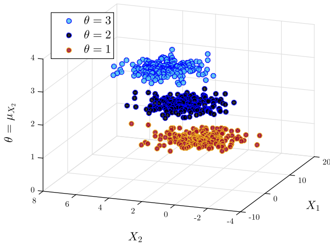
(a) NRA (200 points/cloud, indeed 600 points in total).
