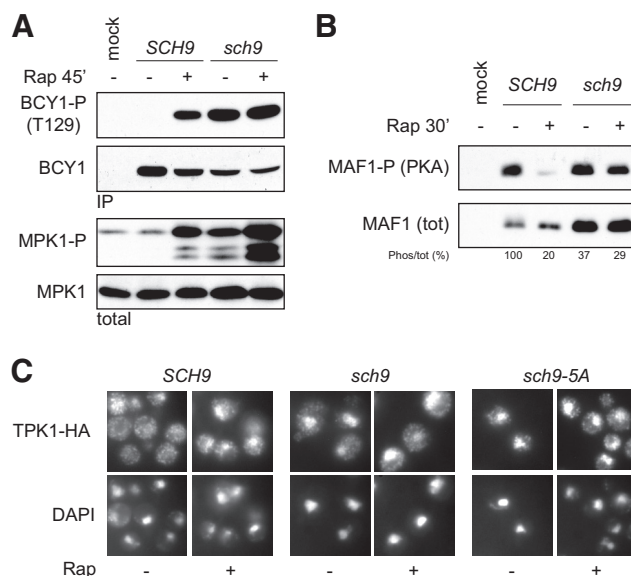
Figure 5. TORC1 inhibits MPK1 and BCY1 T129 phosphorylation through the AGC kinase SCH9. (A) To follow the influence of SCH9 on BCY1 T129 and MPK1 phosphorylation, the yeast strains SA094 ( WT ) and SA135 ( sch9 ) expressing HA-BCY1 were grown to exponential phase and treated 45 min with rapamycin (+) or drug vehicle (-) before total protein extraction. HA-BCY1 was immunoprecipitated (IP) and analyzed by Western blot with anti-HA (HA-BCY1) and anti-RxxS/T [BCY1-P (T129)] antibodies (IP panel). Total (MPK1) and activated MPK1 (MPK1-P) were visualized in total cell lysate by Western blot with the corresponding antibodies (panel total). (B) Effect of SCH9 deletion on PKA-dependent phosphorylation of MAF1. The yeast strains SA148 ( MAF1-HA SCH9 ) and SA232 ( MAF1-HA sch9 ) were grown to exponential phase and treated for 30 min with rapamycin (+) or drug vehicle (-) before total protein extraction. MAF1-HA was immunoprecipitated and analyzed by Western blot with anti-HA [MAF1 (tot)] and anti-RRxS/T [MAF1-P (PKA)] antibodies. For each condition, the phosphorylation at PKA sites was quantified, normalized against the level of total protein, and expressed as percentage [Phos/tot (%)]. (C) The rapamycin-dependent localization of yeast strain SA20X carrying a plasmid expressing wild-type SCH9 ( WT = pJU675), no SCH9 ( sch9 = pRS416), or the mutant sch9 5A ( sch9-5A = pJU822). Cells were treated 30 min with rapamycin (+) or drug vehicle (-). TPK1-HA was localized by the use of an anti-HA antibody. The nucleus was observed by DAPI staining (DNA).
