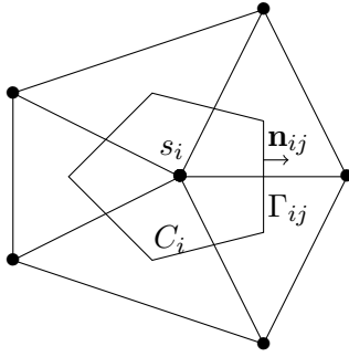
Figure 3: Representation of the dual mesh
