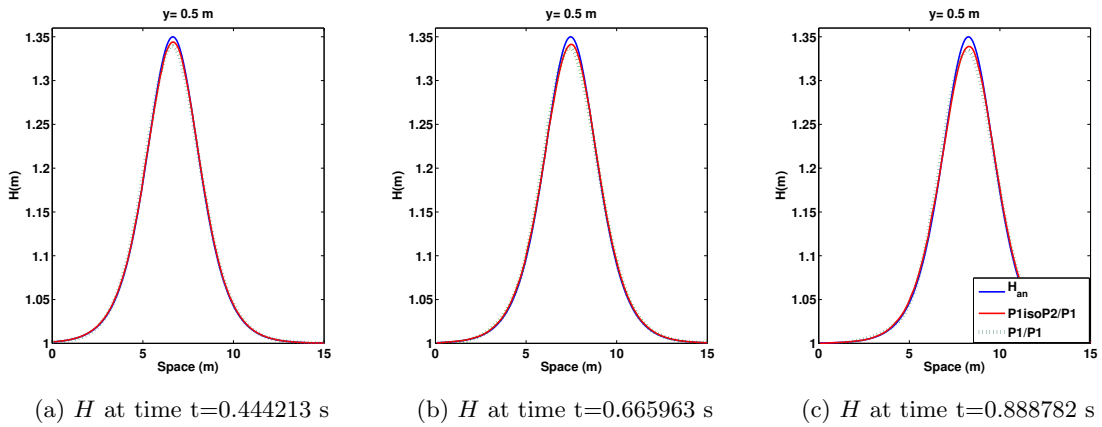
Figure 6: Comparison between the analytical water depth H_{an} and the P_1 iso P_2/P_1 and the P_1/P_1 approximations on the solitary wave propagation.
