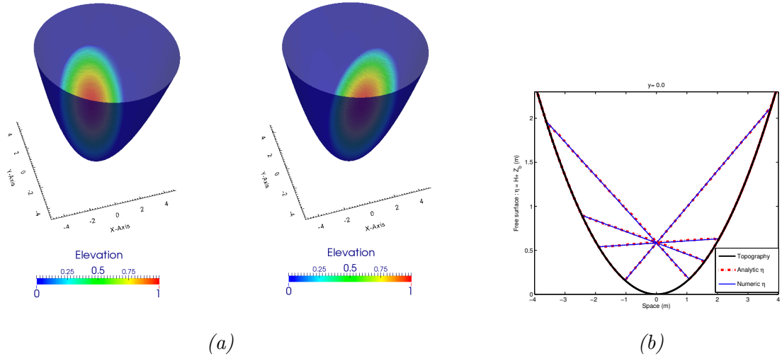
Figure 9: (a) Simulation of the free surface oscillations in a paraboloid at different time steps and (b) cross section of the free surface at y = 0 of the free surface H + z_b compared with the analytical solution at different times: t_0 = 0.277222 s, t_1 = 0.431123 s, t_2 = 0.739382 s, t_3 = 0.893419 s and t_4 = 1.20134 s.
