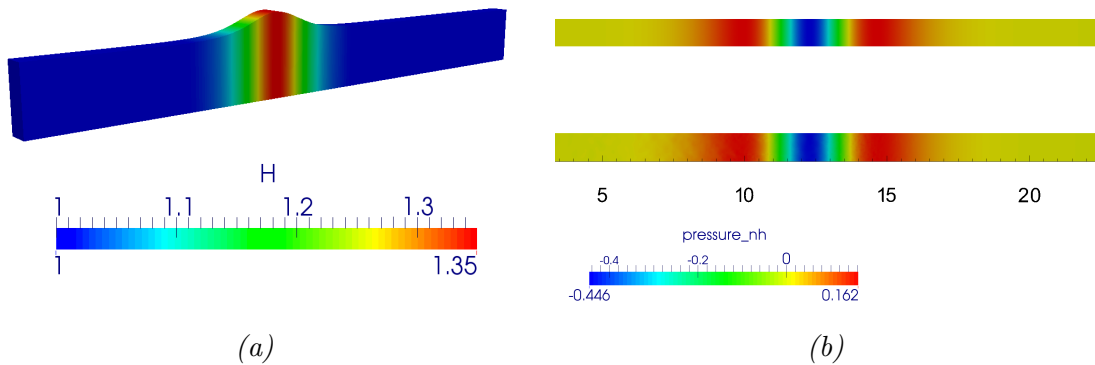
Figure 4: Illustration of the solitary wave propagation at t = 1.99 s, (a) computed water depth (lateral view) and (b) non-hydrostatic pressure (top view), analytical solution at the top, numerical field below.
