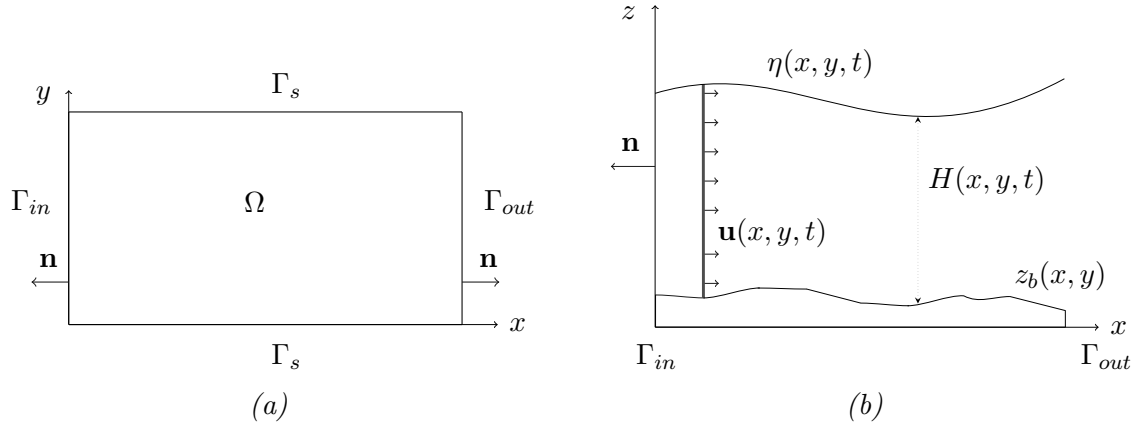
Figure 1: Model domain and notations, (a) view from above and (b) vertical cross section.
