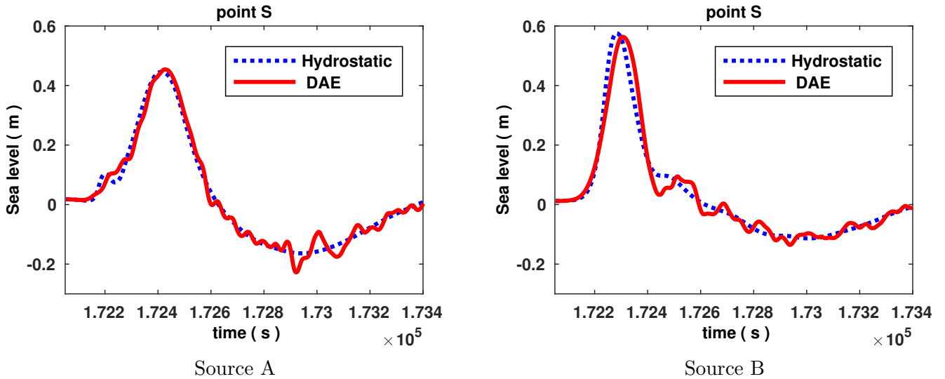
Figure 18: Comparison between numerical results using both models (hydrostatic and non-hydrostatic) at the node S for (a) source A and (b) source B.
