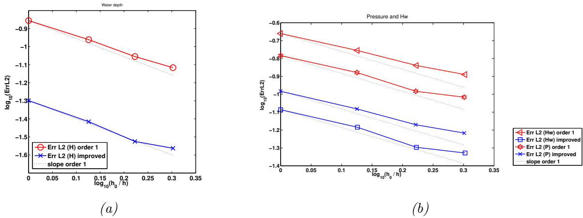
Figure 9: Convergence rate: (a) of the L^2 error of the water depth and (b) of the vertical discharge and the pressure.
