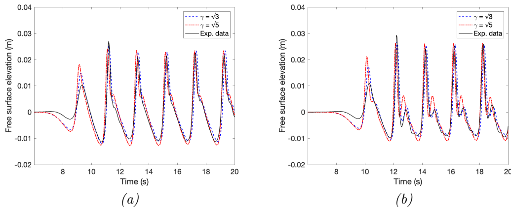
Figure 12: Comparisons between the experimental data (solid line) and the simulations of the dispersive model with \gamma = \sqrt{3} (blue dashed line) and \gamma = \sqrt{5} (red dashed-dotted line). Figs. (a), (b) respectively correspond to the results for the sensors 4 and 5.
