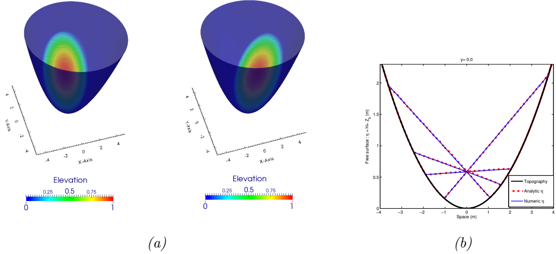
Figure 8: (a) Simulation of the free surface oscillations in a paraboloid at different time steps and (b) cross section of the free surface at y = 0 of the free surface H + z_b compared with the analytical solution at different times: t_0 = 0.277222 s, t_1 = 0.431123 s, t_2 = 0.739382 s, t_3 = 0.893419 s and t_4 = 1.20134 s.
