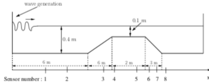
Figure 10: Channel profile for the experiments and location of the sensors.
