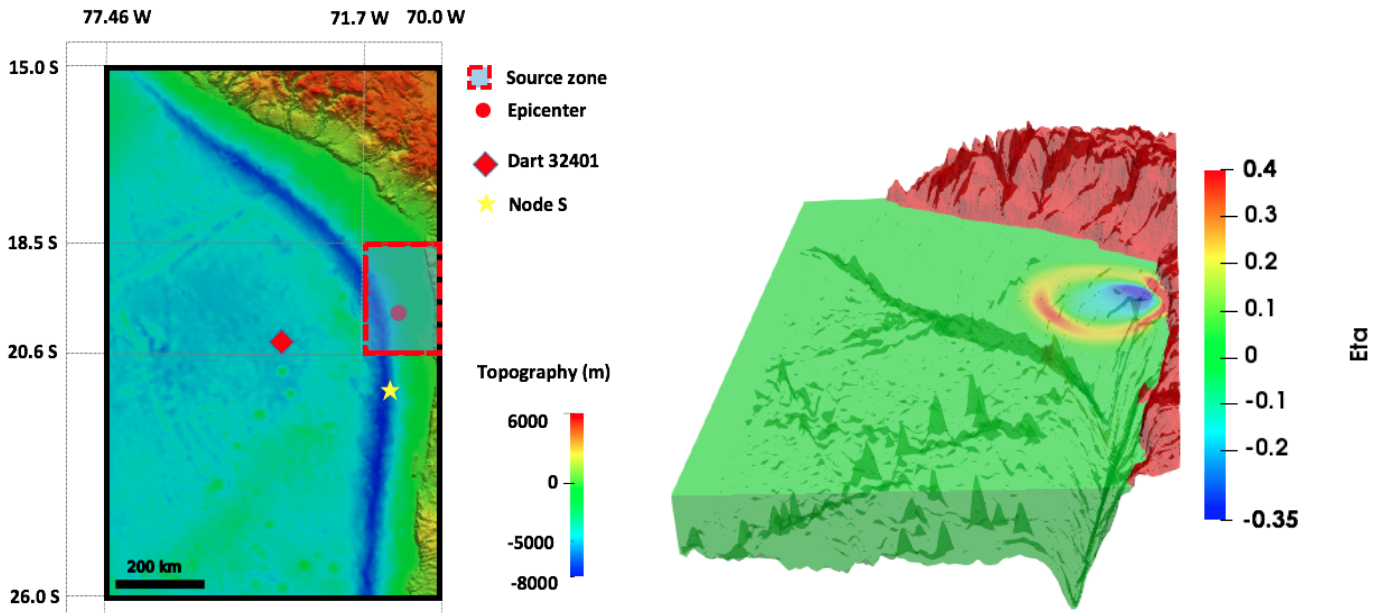
Figure 15: (a) Topography and bathymetry of the simulation domain (Chile) and location of the earthquake epicenter, the DART buoy 32401 and the gauge S. (b) Simulated free surface variation \eta of the tsunami wave at time 666 s.
