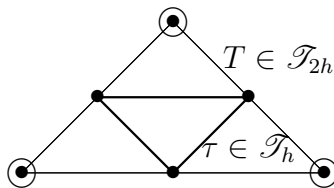
Figure 3: Representation of the triangulation. The velocity is evaluated on the black nodes, while the pressure is evaluated on the circles.
