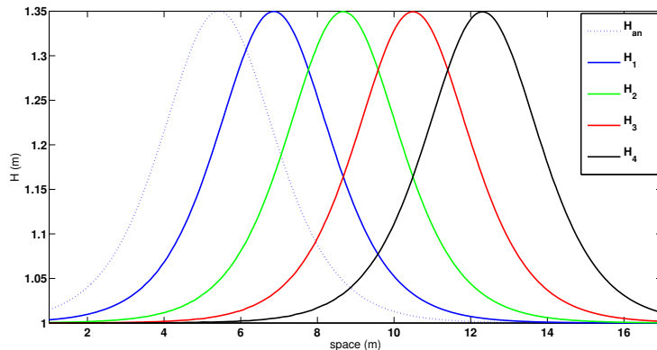
Figure 6: Cross section at the center of the channel y = 0.5 m; water depth of the analytical solution at initial time H_0 = H_{an} and computed solution H(t_i), i = 1, \dots, 4 with t_0 = 0 s, t_1 = 0.499805 s, t_2 = 0.999871 s, t_3 = 1.49983 s, t_4 = 1.99993 s for the P_1 -iso P_2/P_1 approximation and the improved method (Heun scheme).
