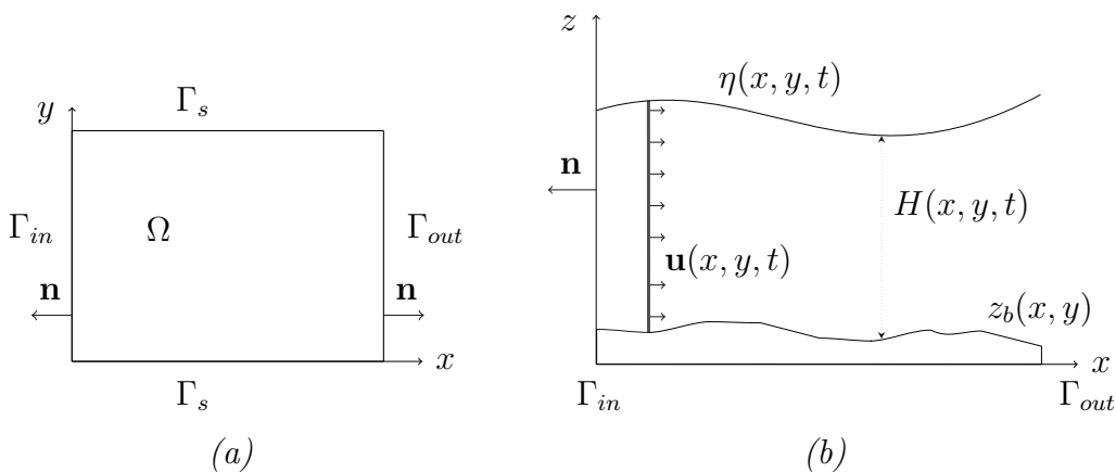
Figure 1: Model domain and notations, (a) view from above and (a) vertical cross section.
