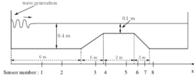
Figure 12: Channel profile for the experiments and location of the sensors.
