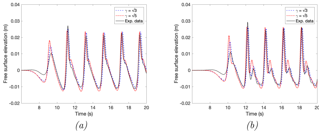
Figure 14: Comparisons between the experimental data (solid line) and the simulations of the dispersive model with \gamma = \sqrt{3} (blue dashed line) and \gamma = \sqrt{5} (red dashed-dotted line). Figs. (a), (b) respectively correspond to the results for the sensors 4 and 5.
