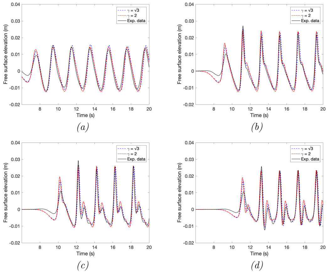
Figure 13: Comparisons between the experimental data (solid line) and the simulations of the dispersive model with \gamma = \sqrt{3} (blue dashed line) and \gamma = 2 (red dashed-dotted line). Figs. (a), (b), (c) and (d) respectively correspond to the results for the sensors 3, 4, 5 and 6.
