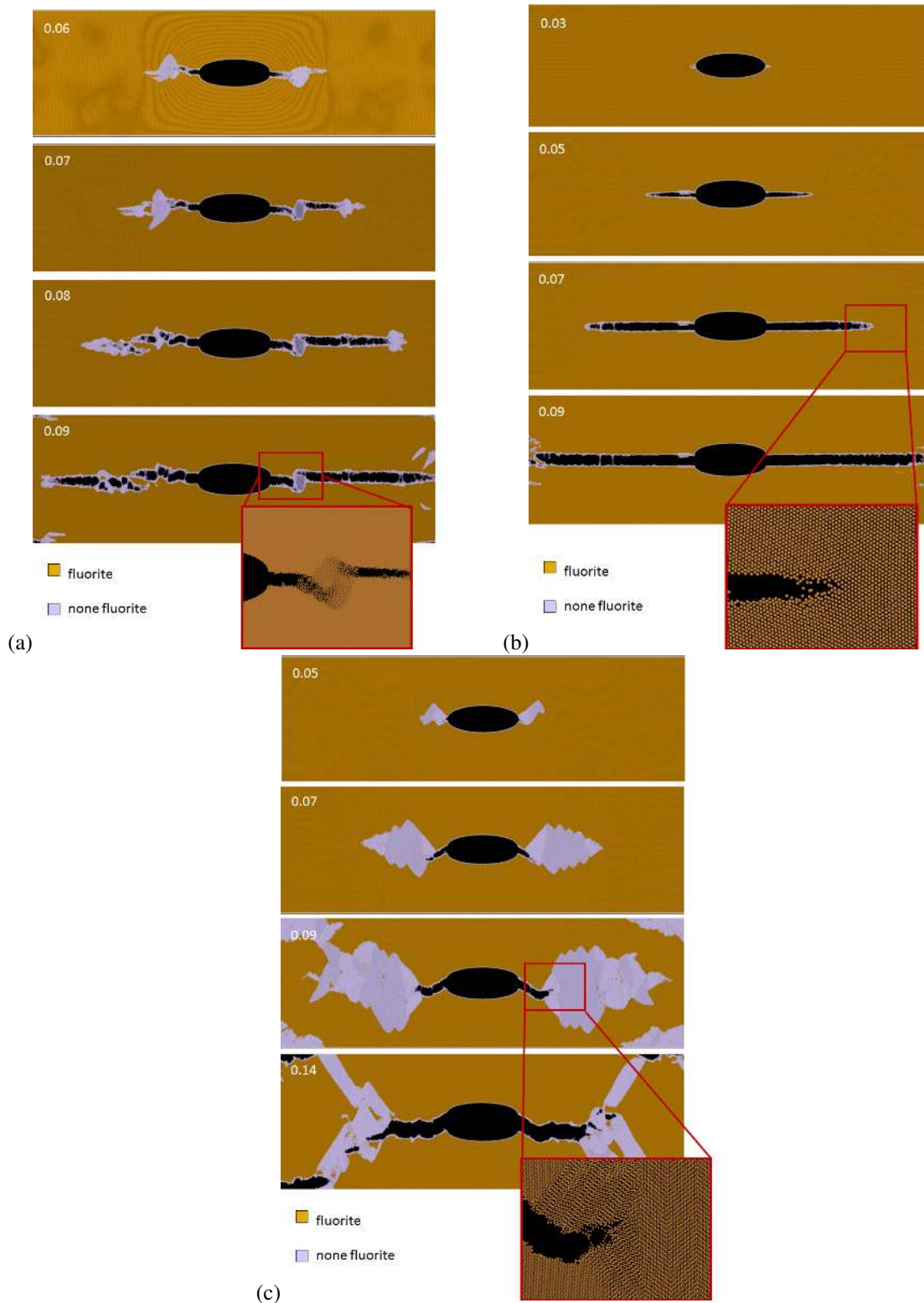
Figure 8: Snapshots during crack propagation in (U,Pu)O_2 system with 25 at.% of plutonium at 300 K for (a) Arima, (b) Potashnikov, and (c) Cooper potentials. The load is applied along the \langle 1\ 1\ 1 \rangle crystallographic direction in the fluorite structure. The inserts in each figure depict a close up of the crack front where phase transition occurs.
