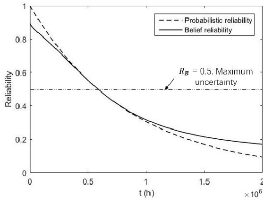
Fig. 9. Belief reliability of the SBC
