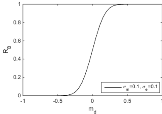
Fig. 2. Influence of m_d on R_B
