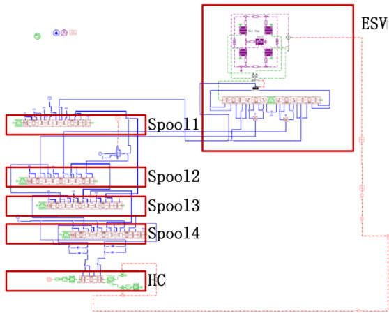
Fig. 7. Schematic of the AMESim model to predict p_{HSA}
