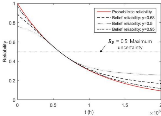
Fig. 10. Belief reliability of the SBC
