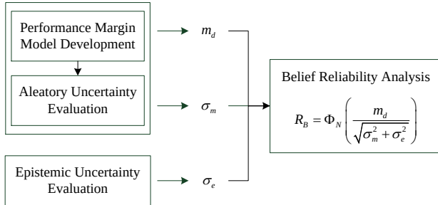
Fig. 5. Procedures for component belief reliability evaluation
