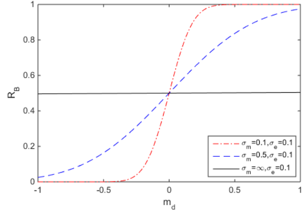
Fig. 3. Variation of R_B with \sigma_m
