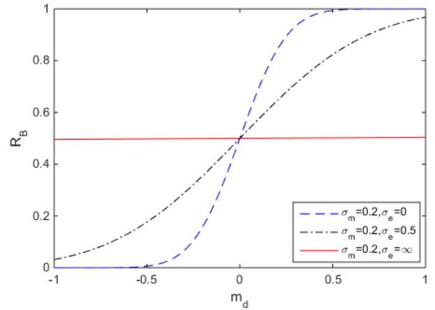
Fig. 4. Variation of R_B with \sigma_e
