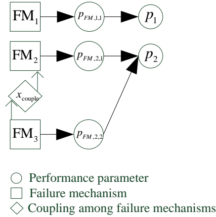
1 2 Figure 5 A illustration of interaction graph
