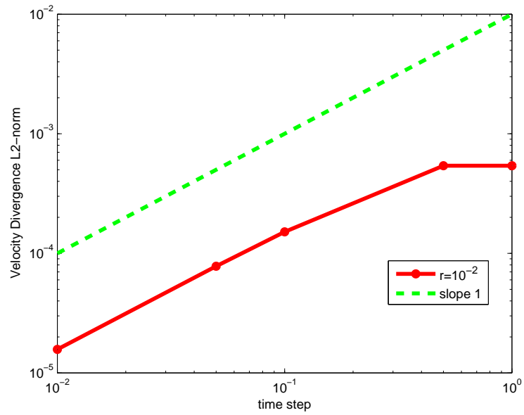
FIGURE 10. Stokes problem - Velocity divergence L^2 -norm versus time step at T=2 , mesh size 1/h = 128 and \epsilon=10^{-6} .
