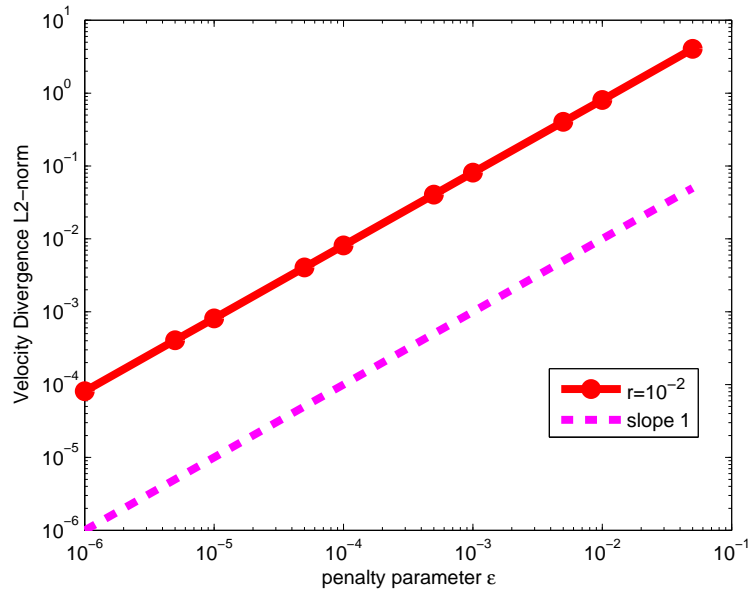
FIGURE 9. Stokes problem - Velocity divergence L^2 -norm versus \epsilon at T=2 , mesh size 1/h = 128 and r = 10^{-2} .
