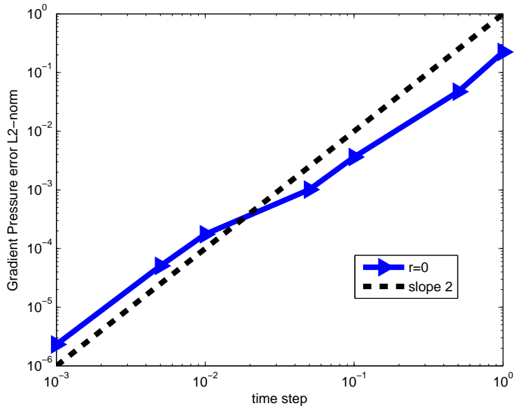
FIGURE 4. Stokes problem - Error on the gradient pressure in L^2 -norm vs \delta t at T = 2 , mesh size 1/h = 128 , \varepsilon = 10^{-10} and r = 0 .
