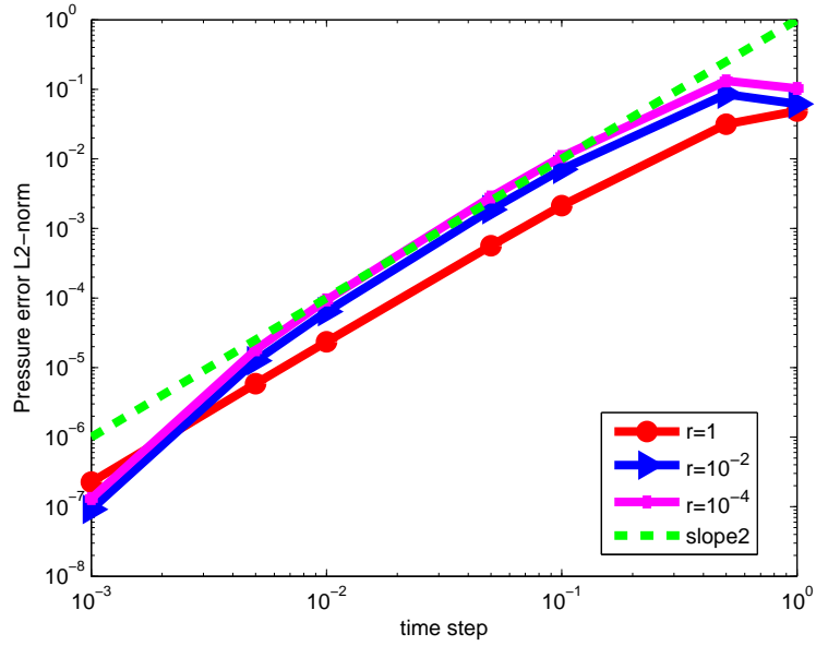
FIGURE 6. Stokes problem - Error on the pressure in L^2 -norm vs \delta t at T = 2 , mesh size 1/h = 128 and \varepsilon = 10^{-10} .
