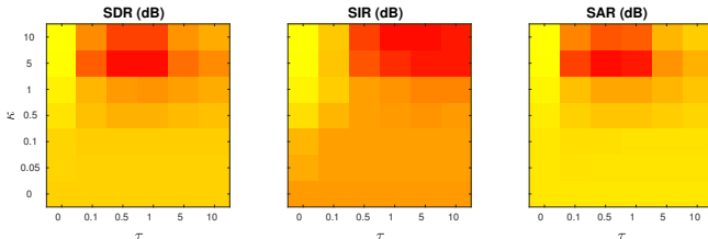
Fig. 2. Influence of the phase parameters \kappa and \tau on the source separation quality. Darker is better.
