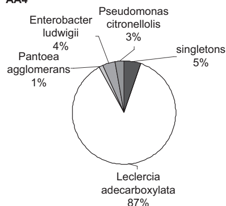
Fig. 4. Identification of representative groups of clones detected in, respectively, Z4 and AA4. Z4 represents families of microorganisms found in the sediment. AA4 represents species of microorganisms (all \gamma proteobacteria) found in the enrichment.
