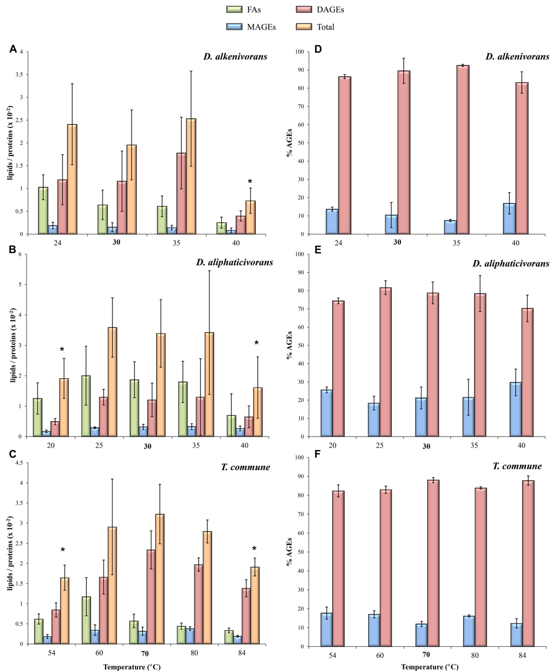
FIGURE 1 | Hydrolyzed lipid content (A–C) and relative abundances of MAGEs and DAGEs (D–F) in the mesophiles D. alkenivorans and D. aliphaticivorans and the thermophile T. commune grown at different temperatures. Data are means of three independent cultures. Optimal growth temperatures are bolded. The asterisks indicate significant differences compared to optimal temperature as determined by the Student's t -test ( p -value < 0.05).
