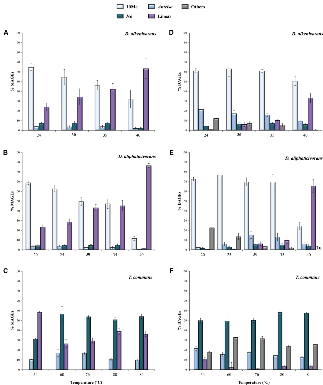
FIGURE 3 | Relative abundances (%) of total) of 10Me, anteiso, iso, and linear MAGEs (A–C) and DAGEs (D–F) released by cell hydrolysis of the mesophiles D. alkenivorans and D. aliphaticivorans and the thermophile T. commune grown at different temperatures. For all strains, “others” correspond to (tentatively identified) DAGEs with two methyl branches at different positions. Each data point is the mean of three independent cultures. Optimal growth temperatures are bolded.
