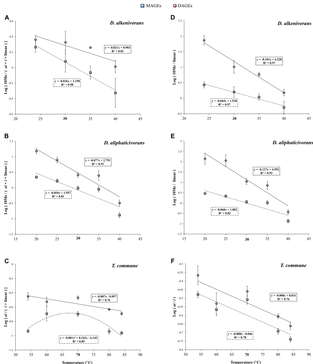
FIGURE 4 | (A,B) Logarithm of the ratios of 10Me to anteiso + iso + linear MAGEs (squares) and monomethyl branched DAGEs (circles) in the mesophiles D. alkenivorans and D. aliphaticivorans vs growth temperature. (C) Logarithm of the ratio of anteiso to iso + linear MAGEs (squares) and DAGEs (circles) in the thermophile T. commune vs growth temperature. (D,E) Logarithm of the ratio of 10Me branched to linear MAGEs (squares) and monomethyl branched DAGEs (circles) in D. alkenivorans and D. aliphaticivorans vs growth temperature. (F) Logarithm of the ratio of anteiso to iso MAGEs (squares) and DAGEs (circles) in T. commune vs growth temperature. Each data point is the mean of three independent cultures. For T. commune , the ratios do not include (tentatively identified) DAGEs with two methyl branches at different positions ( ai/i , i/ai ; see Supplementary Table S1). Optimal growth temperatures are bolded.
