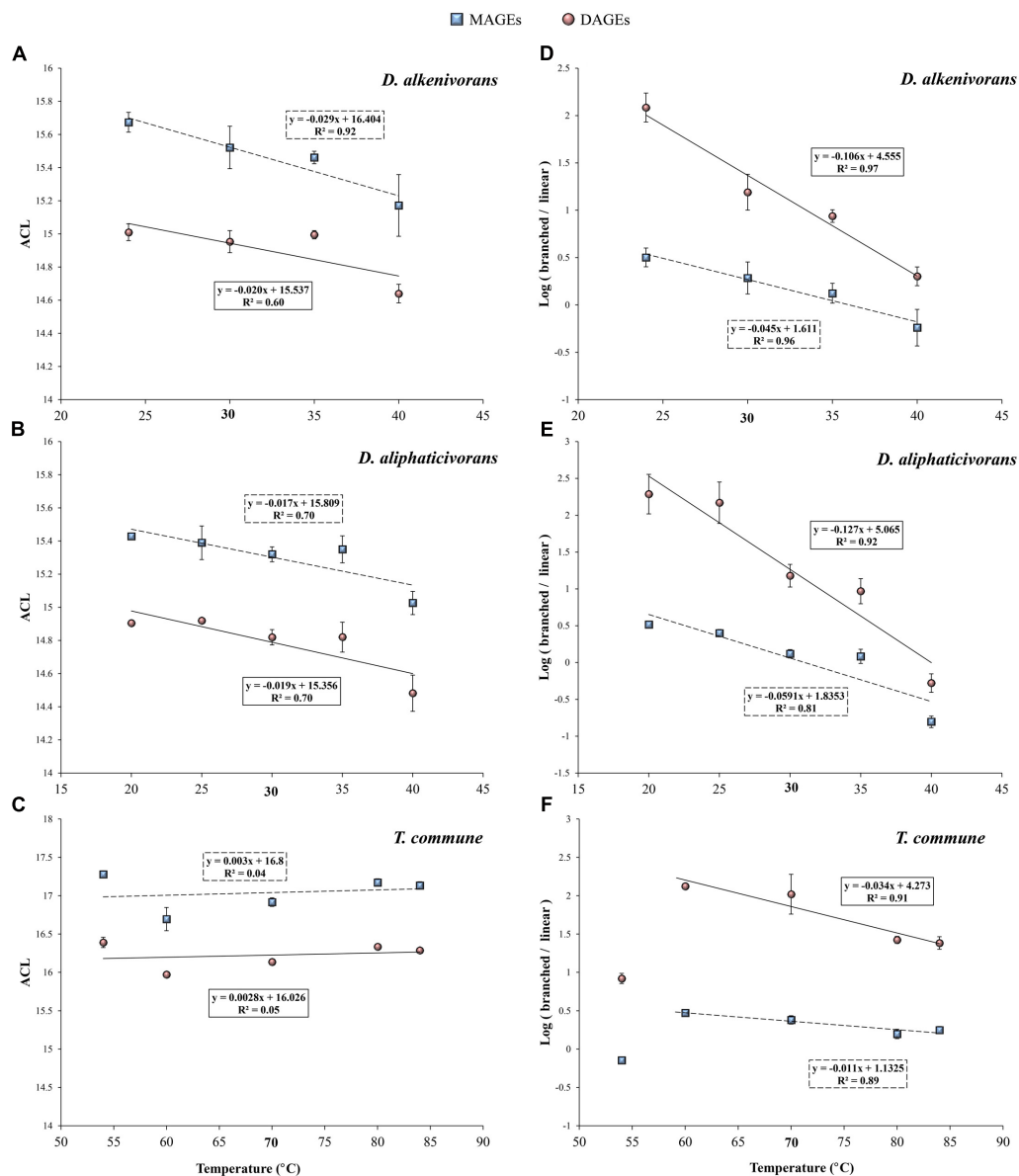
FIGURE 2 | Weighted average chain length (ACL) (A–C) and logarithm of the ratio of branched to linear structures (D–F) of MAGEs and DAGEs formed by the mesophiles D. alkenivorans and D. aliphaticivorans and the thermophile T. commune as a function of growth temperature. Branched DAGEs correspond to all compounds with one or two branched alkyl chain(s) whereas linear DAGEs correspond to unbranched compounds (see Supplementary Table S1 and Figure S2). Each data point is the mean of three independent cultures. Optimal growth temperatures are bolded.
