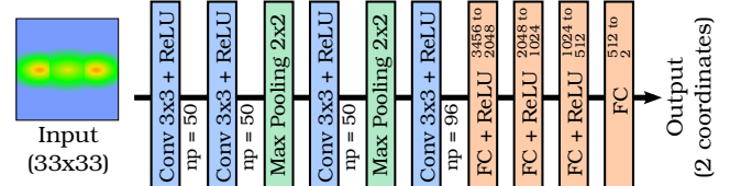
Figure 5: Our CNN architecture for normal estimation.
