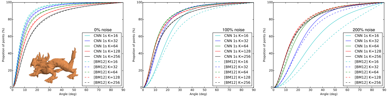
Figure 12: Proportion of normals with error less than a given angle, on 250k-point dragon with noise 0% (left), 100% (middle), 200% (right).
