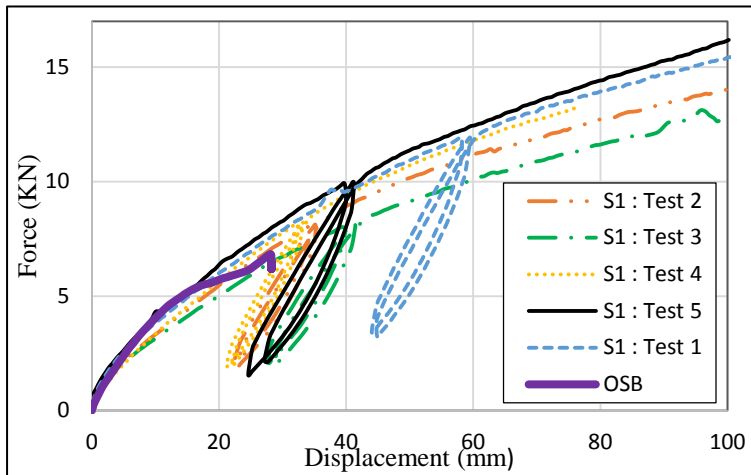
Figure 3: Force-Displacement behaviour.
