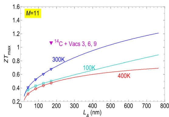
Figure 10. ZT_{max} as a function of the device length for the case of a larger ribbon with M=11 . The open symbols and solid lines are numerical data and fitting curves for the case of 50% isotope doping and 5% vacancies in the m=6 line. The filled symbol is the numerical results of the device with 50% isotope doping and 5% vacancies in lines m=3, 6, 9 .
