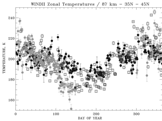
Figure 6. Comparison of WINDII temperature climatological means at 87 km, obtained at 35°N–45°N latitude from 1991 to 1997 (solid circles) with Na lidar temperatures at 87 ± 2.4 km at Fort Collins (41°N, 255°E) from 1990 to 1999 (squares) (courtesy C. Y. She), and OH rotational temperature climatology at 87 km at Bear Lake Observatory (42°N, 212°E) from 1991 to 1996 (shaded circles) (courtesy P. J. Espy).
