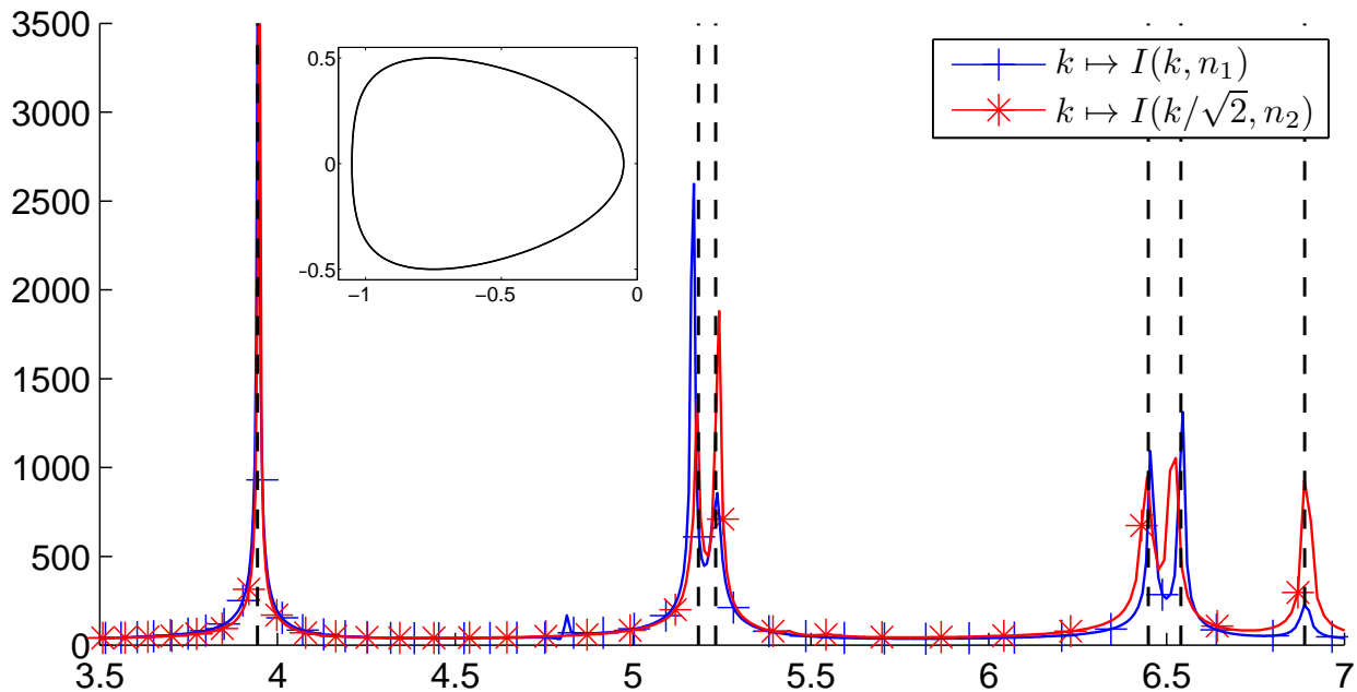
Figure 1 – Curves k \mapsto I(k, n_1) and k \mapsto I(k/\sqrt{2}, n_2) for k \in (3.5; 7) . The vertical dashed lines correspond to the eigenvalues of Problem (9) computed with n = n_1 in \Omega (the quantities we want to retrieve in practice). The kite shaped domain represents the inclusion \Omega .
