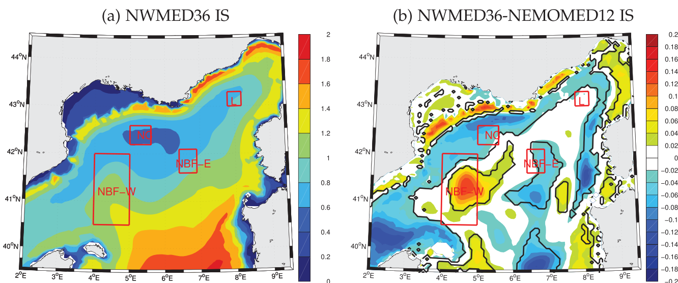
Figure 8. (a) NWMED36 time mean bottom Index of Stratification (IS, m^2/s^2 ) for the period 1 August 2012 to 30 June 2013. (b) NWMED36 time mean bottom IS anomaly map with respect to NEMOMED12. The black contour displays the 99% significance level (Student's t test, two sided) for ensemble mean differences. The areas where dense water formation differs are displayed in red: the Northern Current (NC), Western (NBF-W) and Eastern (NBF-E) North Balearic Front, and the Ligurian Sea (L).
