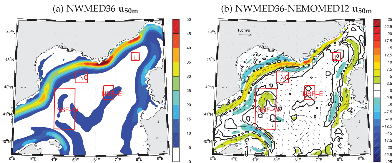
Figure 7. (a) NWMED36 time mean velocities at 50 m depth ( u_{50} , cm/s) and their module ( |u_{50}| ) for the period 1 August 2012 to 30 June 2013. (b) NWMED36 time mean u_{50} anomaly map with respect to NEMOMED12. The black contour displays the 99% significance level (Student's t test, two-sided) for ensemble mean differences. The four areas where dense water formation differs are displayed in red: the Northern Current (NC), Western (NBF-W) and Eastern (NBF-E) North Balearic Front, and the Ligurian Sea (L).
