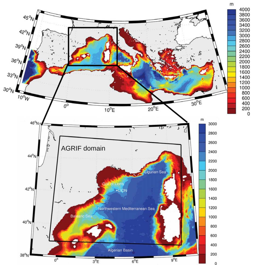
Figure 1. (top) Domain and associated bathymetry for NEMOMED12 and (bottom) its embedded NWMED36 configuration in the northwestern Mediterranean Sea. The locations of LION buoy and the main basins are displayed.
