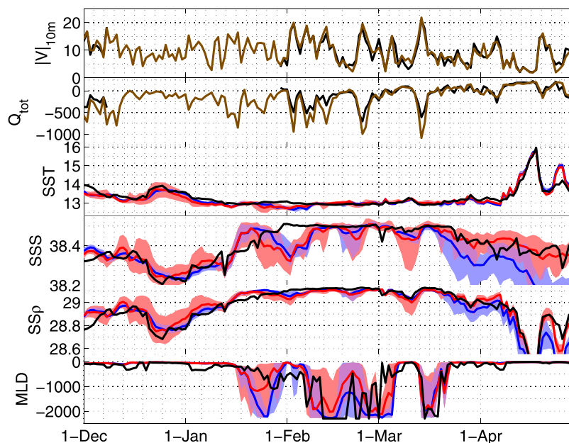
Figure 3. In the plot, black lines represent LION buoy/mooring data, brown ALDERA forcing, blue and red show, respectively, NEMOMED12 and NWEMED36 simulation ensembles (ensemble mean, minimum, and maximum). From top to bottom: daily time series of near-surface wind |V|_{10m} and net surface heat flux Q_{tot} , sea surface temperature (SST), salinity (SSS) and density ( SS\rho ) and mixed layer depth (MLD) at LION location between 1 December 2012 and 30 April 2013.
