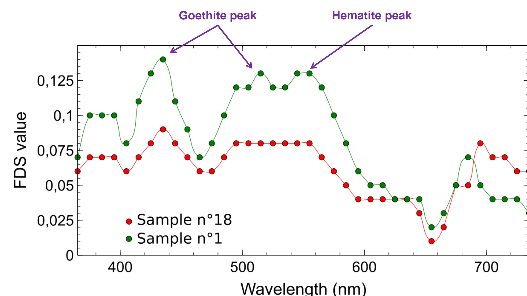
Fig.3 Variations of the FDS value in the Canche watershed: example for sample n°1 and n°18. Spectral reflectance were measured between 360 and 740 nm with a 10-nm resolution
