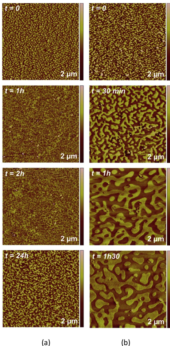
Fig. 3. AFM tapping mode phase 2 \times 2 \mu\text{m}^2 images of a 45 nm thickness film of \text{SBM}_{T+D+Aox} : (a) annealed under vacuum at 120 °C for 24 h, (b) annealed at 120 °C for 1 h 30 min under ventilated oven.
