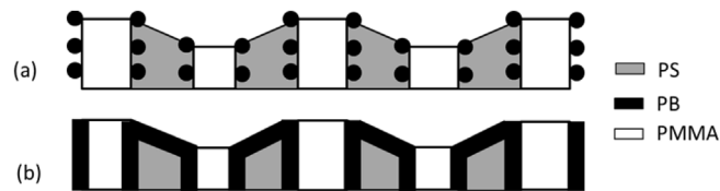
Fig. 2. “Ball at the wall” morphology (a) proposed by Stadler [12,13] for a SBM having weight fractions w_{\text{PS}} = 0.45 , w_{\text{PB}} = 0.06 , w_{\text{PMMA}} = 0.49 , (b) proposed for the SBM studied in this work with higher PB content.
