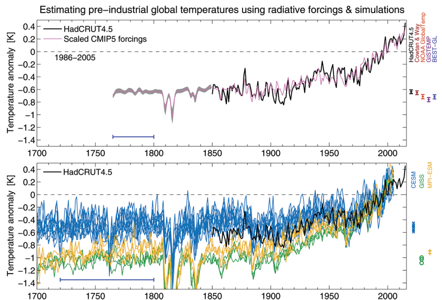
FIG. 2. (top) Estimating global preindustrial temperature using scaled radiative forcings (pink), using HadCRUT4 (black) as the reference. The gray shading represents the uncertainty in the regression. Estimated global temperature anomalies for 1765–1800 are given for all five global temperature datasets (right-hand side, as labeled). (bottom) Simulated global temperature anomalies in the LMEs and estimates for the change since 1720–1800 for the range of ensemble members of CESM (blue), GISS (green), and MPI-ESM (orange). In both panels the blue horizontal bars indicate the period used for averaging. Temperature anomalies are presented relative to the mean of the reference period 1986–2005 (dashed black line).
