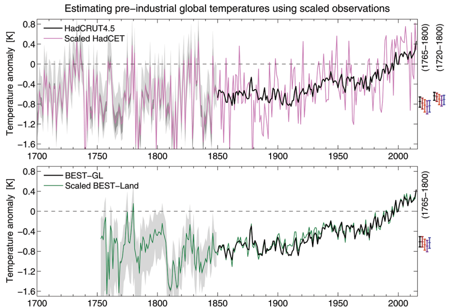
FIG. 3. Estimating global preindustrial temperature using scaled annual-mean observations for (top) CET scaled to HadCRUT4 and (bottom) BEST-Land scaled to BEST-GL, relative to 1986–2005 (dashed black). The dark gray shading (hardly visible) represents the uncertainty in the regressions and the light gray shading the uncertainty in the observations. The sets of five error bars on the right-hand side use the different global temperature datasets, with the same ordering as in the top panel of Fig. 2, for the two different averaging periods as labeled. Note the vertical scale is different from Fig. 2.
