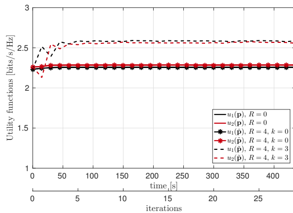
Fig. 6. Utility functions of the players - Low interference, d_{ji}/d_{ii} = 3 , d_{ii} = 1 km.
