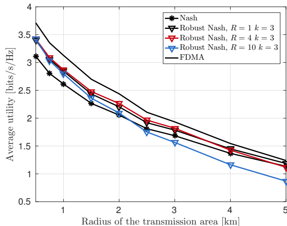
Fig. 8. Influence of the estimators quality on the robust games. Two players, reference SNR = 20 dB at 1 km.
