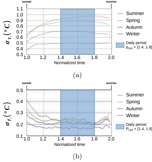
Figure 2: Mean night-time temperature dispersion (a) and mean night-time cooling rate dispersion (b) for each season represented along a normalized time axis
