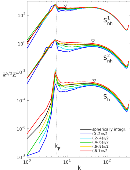
Figure 18. Directional energy spectra E_i(k) for runs in set S. Markers indicate the Zeman scale k_\Omega = \sqrt{(2\Omega)^3/\epsilon} .
