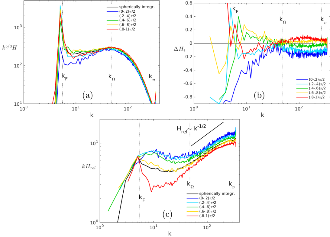
Figure 20. (a) Directional helicity spectra H(k, \theta) compensated by k^{5/3} , (b) helicity directional anisotropy \Delta H_i(k) , (c) relative helicity directional spectra H_{rel_i}(k) = H_i(k) / (2kE_i(k)) , for run S_h .
