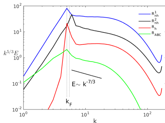
Figure 13. Spherically averaged energy spectra E(k) compensated by k^{5/3} , for runs in set R.
