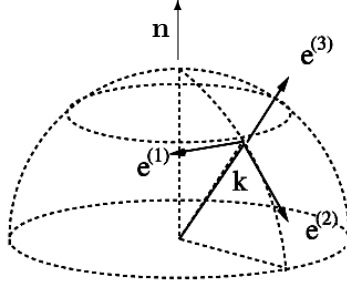
Figure 1. Craya-Herring frame of reference.
