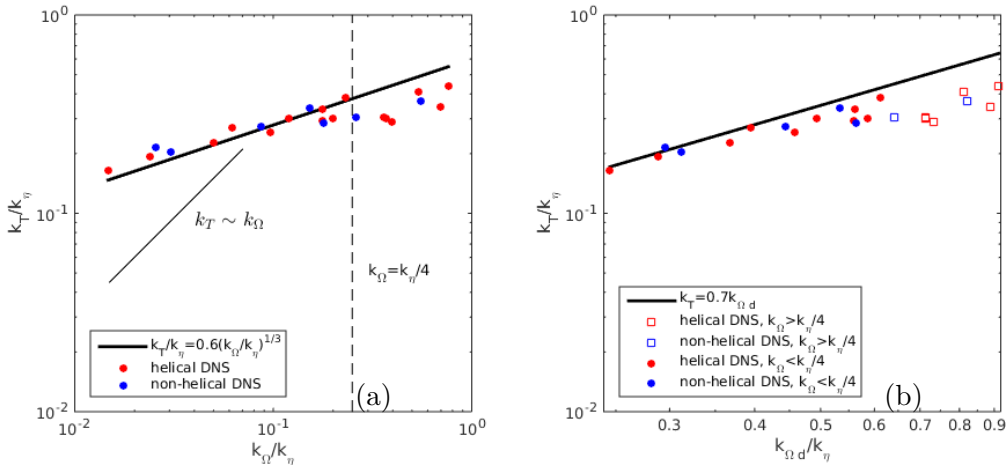
Figure 22. k_T/k_\eta plotted as a function of (a) k_\Omega/k_\eta , (b) k_{\Omega d}/k_\eta . For comparison, the slope corresponding to k_T \sim k_\Omega is shown too.
