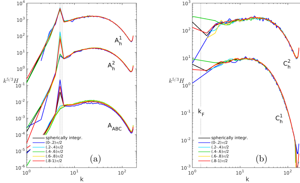
Figure 9. Directional helicity spectra H_i(k) compensated by k^{5/3} for: (a) runs A_h^1 , A_h^2 and A_{ABC} ; (b) runs C_h^2 and C_h^1 .
