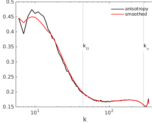
Figure 21. Anisotropy indicator (defined by Eq. (15)) for run S_{\text{nh}}^2 .
