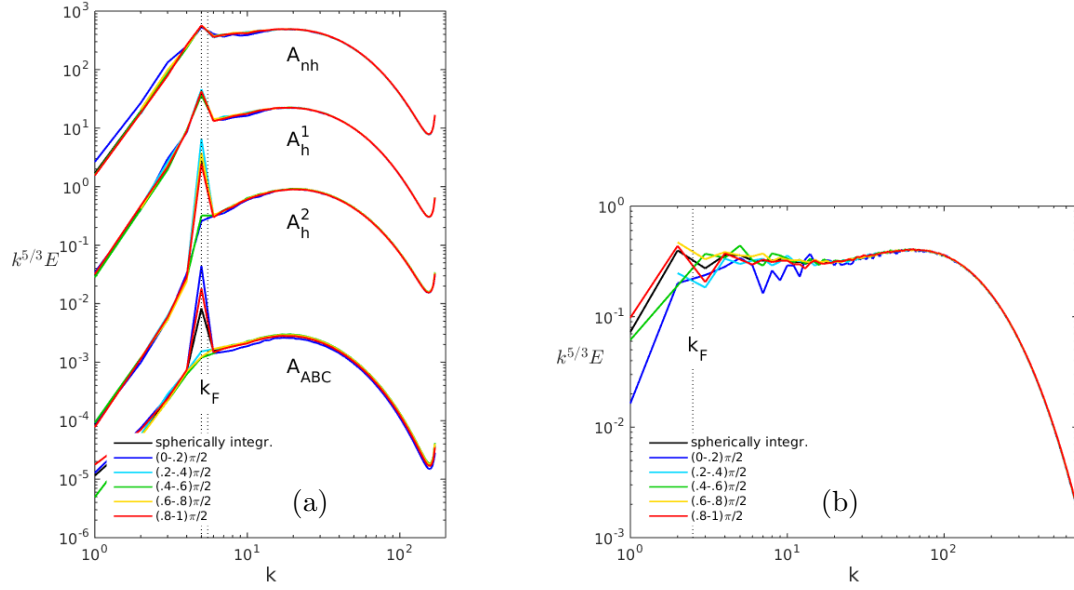
Figure 4. Directional energy spectra E_i(k) compensated by k^5/3 , as functions of wavenumber k for the five angular sectors for: (a) set A ( k_F = 5, 5.5 ); (b) run D_{nv} . The five sectors are indicated in legend, and the same colorcode applies throughout the paper.
