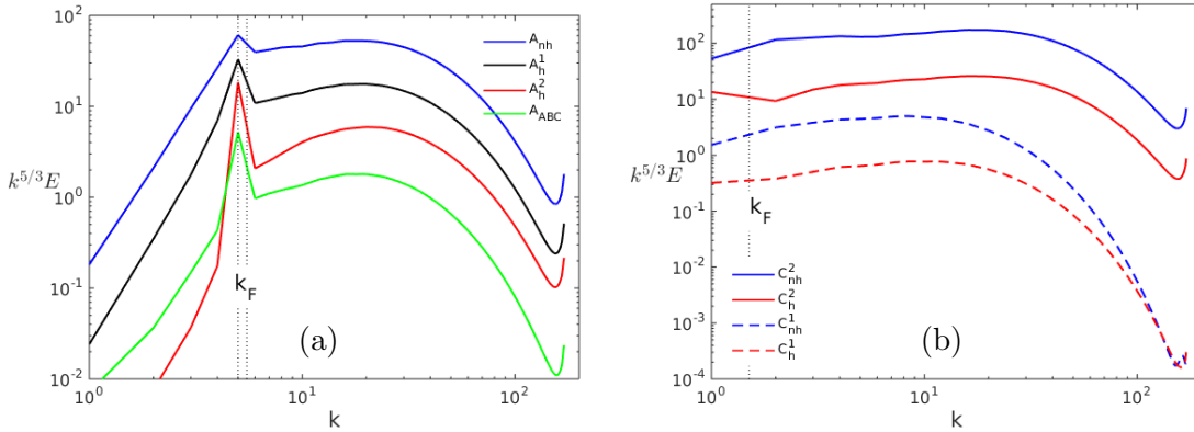
Figure 3. Spherically integrated kinetic energy spectra: (a) for runs in set A ( k_F \simeq 5 ); (b) for runs in set C ( k_F = 1.5 ). Spectra are shifted vertically for better view, and are compensated by the Kolmogorov inertial scaling k^{5/3} . k_F indicates the forcing wavenumber, as in the following plots.
