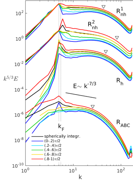
Figure 14. Directional energy spectra E_i(k) , compensated by k^{5/3} for runs in set R. Markers indicate the Zeman scale k_\Omega = \sqrt{(2\Omega)^3 / \epsilon} .
