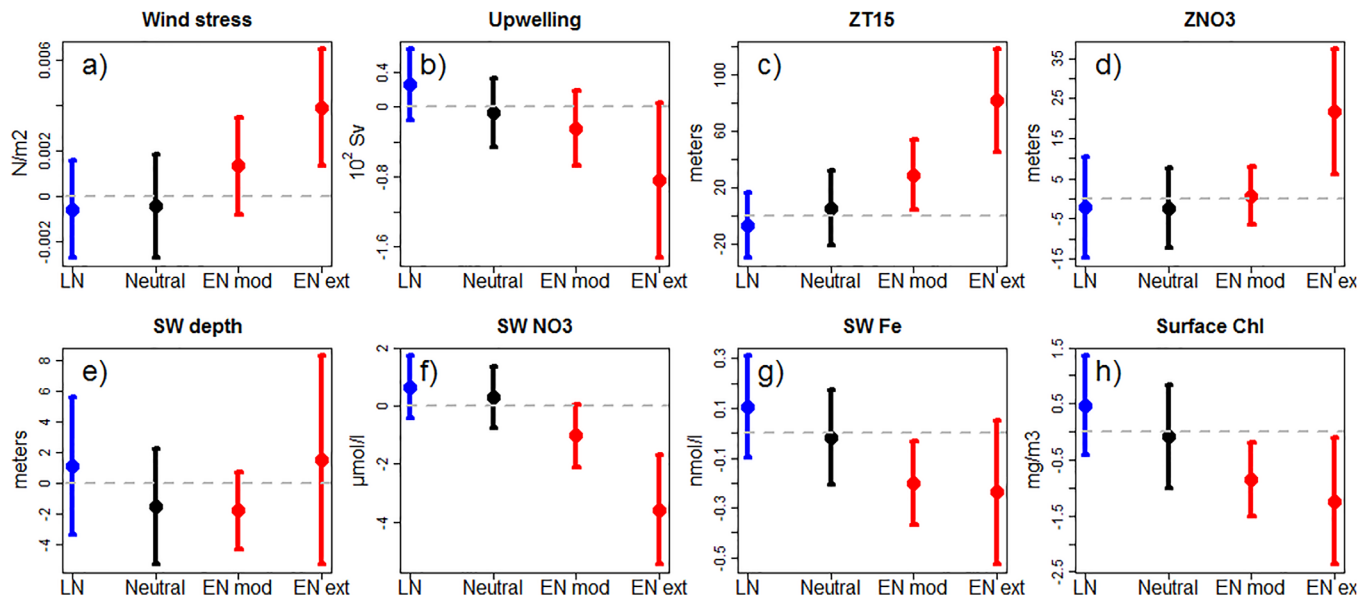
Figure 13. (a) Wind stress (in N.m^{-2} ), (b) upwelling rate (in 10^2 Sv ), (c) ZT (in meters), (d) ZNO 3 (in meters), (e) SW depth (in meters), (f) SW nitrate concentration (in \mu mol.L^{-1} ), (g) SW iron concentration (in nmol.L^{-1} ), and (h) Chl concentration (in mg.m^{-3} ) during LN (blue bar), Neutral (black bar), EN moderate and EN extremes (red bars). All variables are averaged in a coastal band (see Figure 1). Error bars represent the standard deviation.
