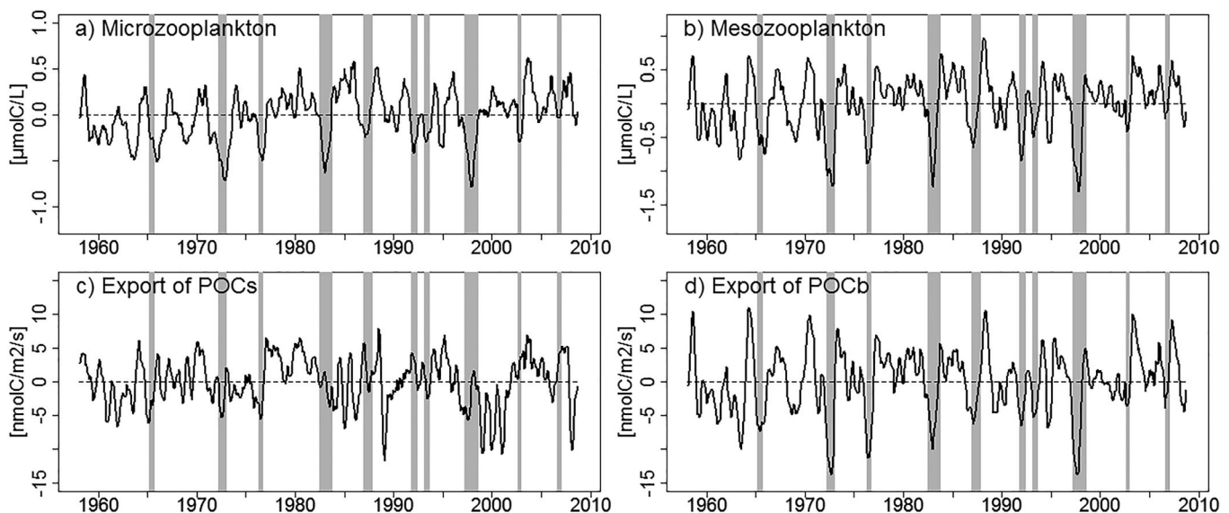
Figure 14. Time series of modelled zooplankton surface concentration (in \mu mol.C.L^{-1} ): (a) microzooplankton and (b) mesozooplankton, (c) small and (d) big POC downward flux (in nmol.C.m^{-2}.s^{-1} ) anomalies. All variables were averaged in a coastal band (see Figure 1) and filtered using a 6 month moving average filter.
