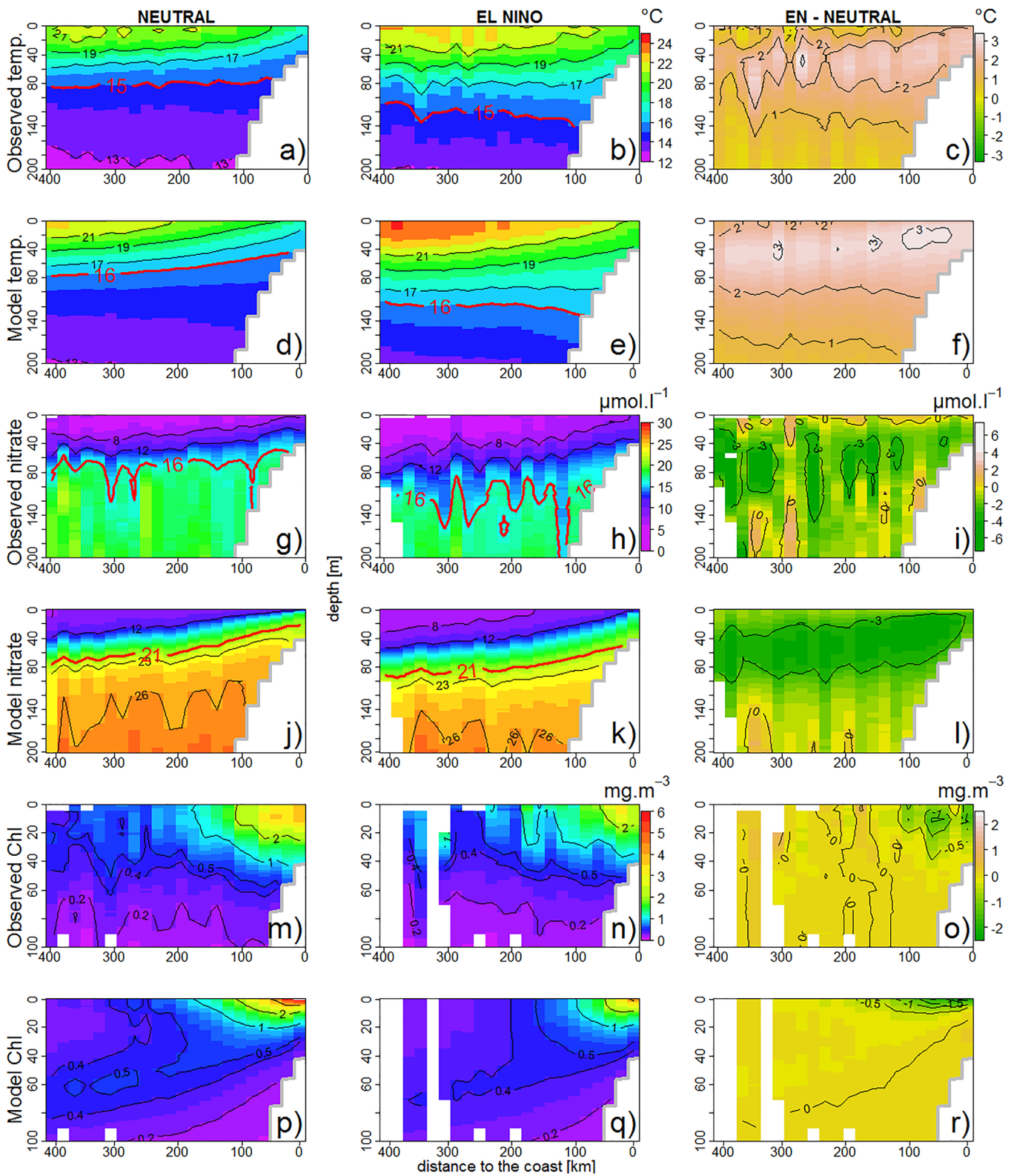
Figure 3. Along-shore averaged vertical section (between 6°S and 16°S) of observational data from IMARPE and model variables: (a–f) temperature ( ^{\circ}\text{C} ), (g–l) nitrate ( \mu\text{mol.L}^{-1} ), and (m–r) chlorophyll ( \text{mg.m}^{-3} ). (left column) Neutral periods, (middle column) El Niño periods, and (right column) differences between EN and Neutral period are shown. Red lines mark ZT (Figures 3a, 3b, 3d, 3e) and \text{ZNO}_3 (Figures 3g, 3h, 3j, 3k).
