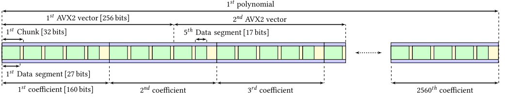
Fig. 3. Software representation of one polynomial of the public key.
