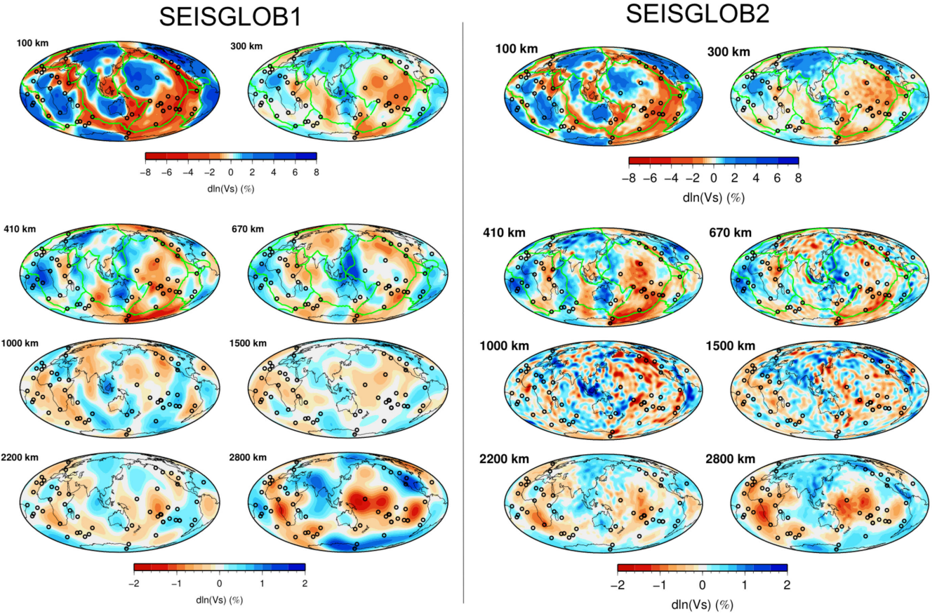
Figure 4. Shear velocity anomalies of SEISGLOB1 (left) and of SEISGLOB2 (right) at various depth with respect to PREM (Dziewonski & Anderson 1981). The green lines show the plate boundaries and black circles the principal hotspots.
