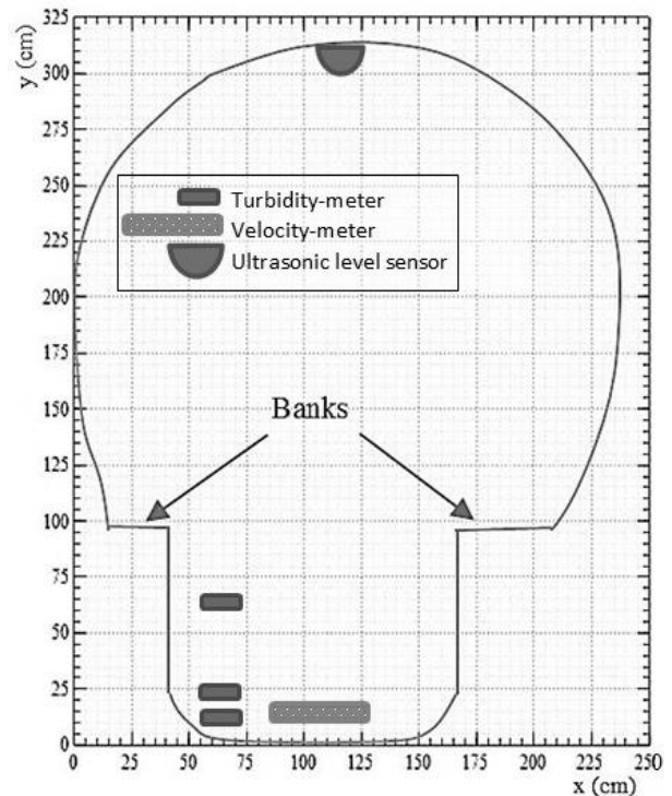
Fig. 1 Sewer Cross-section Details and Measurement Equipment Position
