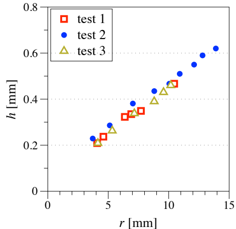
Figure 6: The height versus the radius of the blister as quantified in the experimental measurements in three separate tests for a film thickness t = 850\ \text{nm} . The maximum relative errors for measurements of the height h and radius r of the blister were 2% and 5%, respectively.
