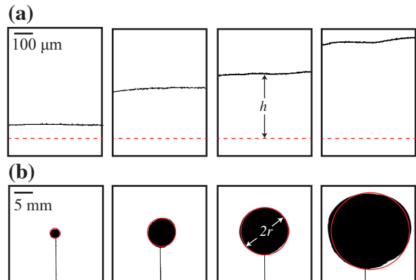
Figure 5: Visualization of the deflection of the film. (a) Side-view visualization of the center of the blister. The dashed red line represents the zero level before the injection of liquid under the PS film. (b) The corresponding top-view images are included to facilitate visualizing the size of the blister.
