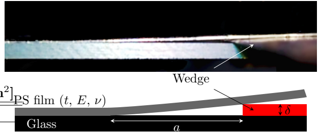
Figure 7: Picture and schematic of the cleavage test of a PS film on a glass slide.
