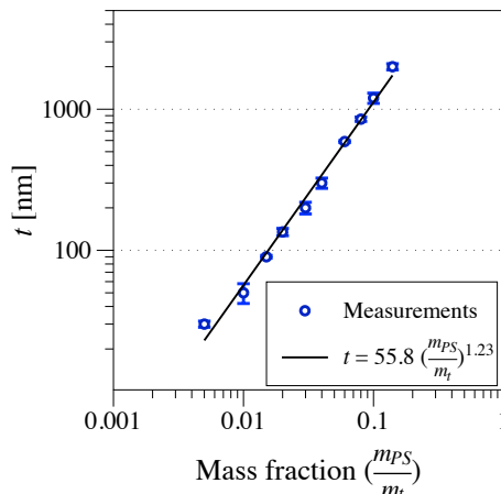
Figure 2: Thickness t of the PS films vs. the mass fraction of PS in toluene used in the spin-coating. Error bars represent the standard deviations of the measurements.
