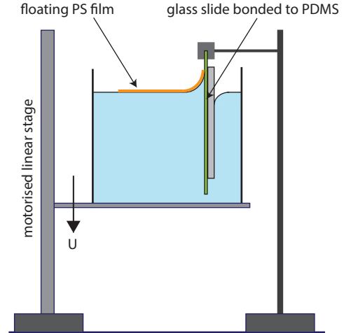
Figure 3: Schematic of the experimental setup for the transfer of the PS film (orange) onto the device.
