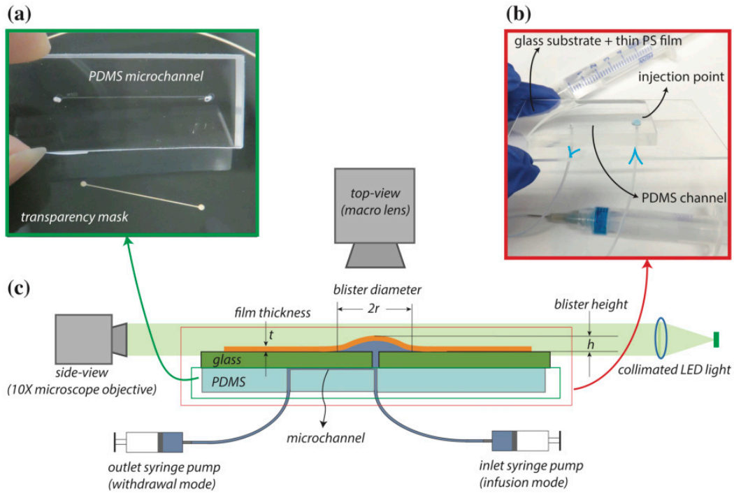
Figure 1: Schematic of the setup for the blister test. (a) A microchannel with a cross-sectional area of 250 \times 250 \mu\text{m}^2 is fabricated in PDMS using a transparency mask and performing soft lithography technique. (b) The inlet of the PDMS microchannel is aligned with the hole drilled in the receiver substrate before the two pieces are bonded together. Finally, the thin PS of thickness t is transferred to the free side of the glass slide to create the blister test device. (c) Dyed water is injected through the inlet underneath the thin film, whilst the trapped air in the hole is evacuated through the outlet of the microchannel. The side-view and top-view images of the blister are captured to determine the maximum deflection h and the diameter 2r of the blister, respectively.
