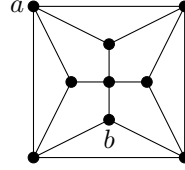
Figure 3: The unique diameter-2 planar graph of domination number 3 [16].
