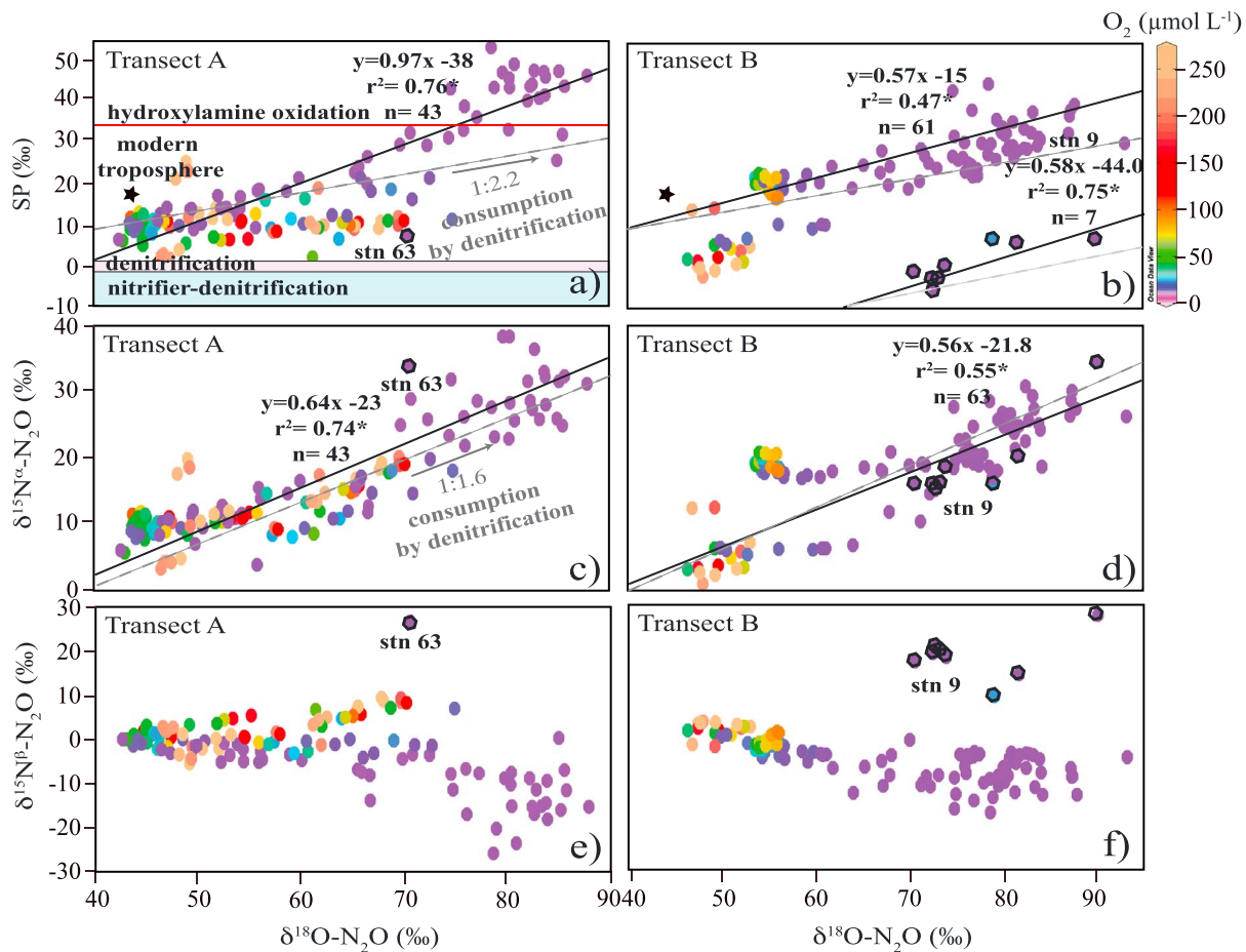
Figure 6. (a and b) SP versus \delta^{18}\text{O-N}_2\text{O} , (c and d) \delta^{15}\text{N}^\alpha\text{-N}_2\text{O} versus \delta^{18}\text{O-N}_2\text{O} and (e and f) \delta^{15}\text{N}^\beta\text{-N}_2\text{O} versus \delta^{18}\text{O-N}_2\text{O} for coastal transects A and B with color-coded [\text{O}_2] (z axis). SP values for \text{N}_2\text{O} production by hydroxylamine oxidation, nitrifier-denitrification, and denitrification as well as for the modern troposphere (black stars [Yoshida and Toyoda, 2000]) are shown in Figures 6a and 6b. The pale grey dashed lines in Figures 6a–6d are the relationships between SP versus \delta^{18}\text{O-N}_2\text{O} and \delta^{15}\text{N}^\alpha versus \delta^{18}\text{O-N}_2\text{O} expected during pure \text{N}_2\text{O} consumption by denitrification. The black lines are the linear regressions for samples with [\text{O}_2] < 5 \mu\text{mol L}^{-1} . Stars next to r^2 values indicate significant relationships. The hexagons are data points from stations 63 (transect A) and 9 (transect B) showing an increase in \delta^{15}\text{N}^\beta\text{-N}_2\text{O} with \delta^{18}\text{O-N}_2\text{O} . Only shelf waters ( <300\text{ m} depth for transect A and <500\text{ m} depth for transect B) were considered.
