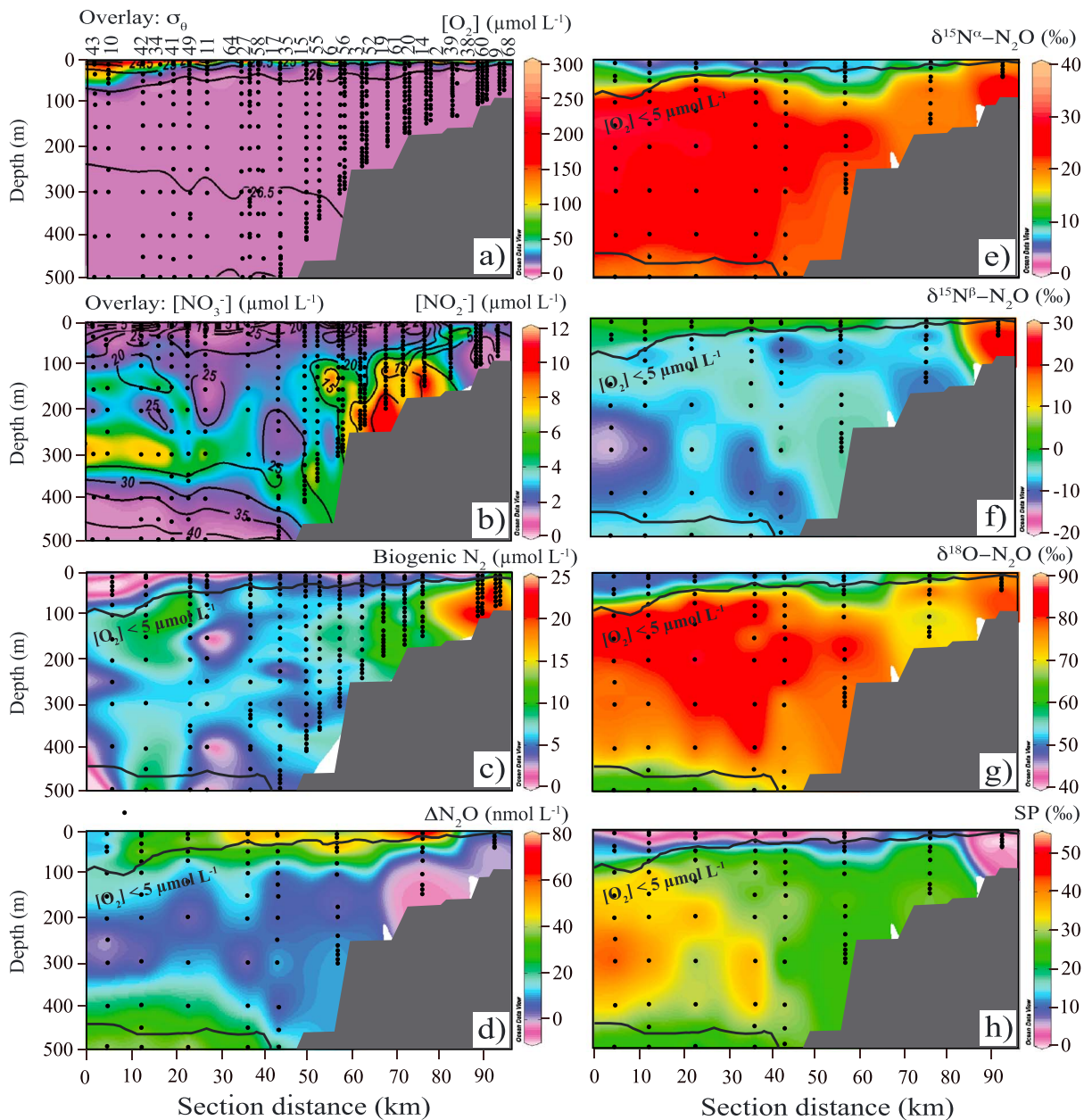
Figure 4. Key parameters for transect B normal to the Peru Coast (see Figure 2). (a) [O_2] with \sigma_\theta in overlay, (b) NO_2^- with [NO_3^-] in overlay, (c) biogenic N_2 (from N_2/Ar data), (d) \Delta N_2O , (e) \delta^{15}N^\alpha-N_2O , (f) \delta^{15}N^\beta-N_2O , (g) \delta^{18}O-N_2O , and (h) SP. CTD numbers are indicated at the top of Figure 4a. Bottom depth was \sim 2000 m at the deepest station 43.
