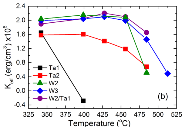
FIG. 1. (a) Schematic drawing of top electrode half-MTJ stack and (b) effective perpendicular anisotropy ( K_{\text{eff}} ) as a function of annealing temperature.
