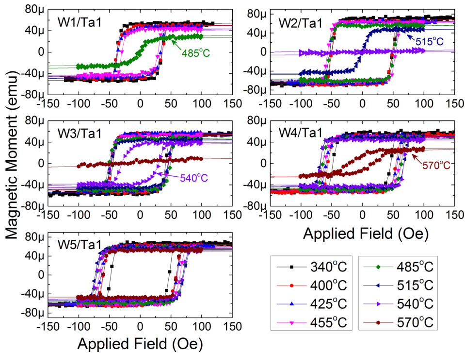
FIG. 2. Out-of-plane M(H) loops of half-MTJs with W (1, 2, 3, 4, and 5)/Ta 1 nm cap as a function of annealing temperature.
